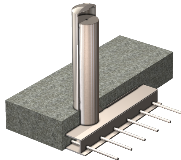
INSTALLED BOLLARD SLEEVE K4M30 Shallow Mounting Shown
