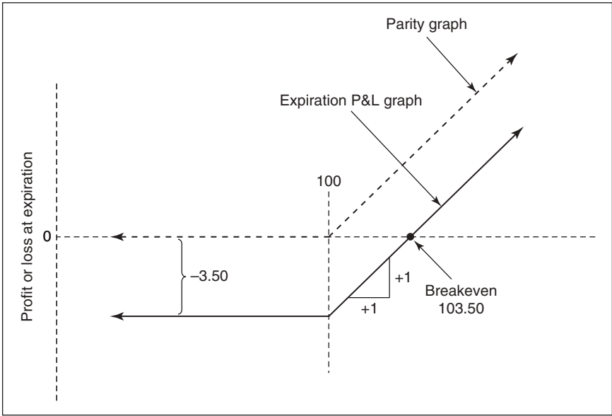
Figure 4-10 Long a 100 call at a price of 3.50.
