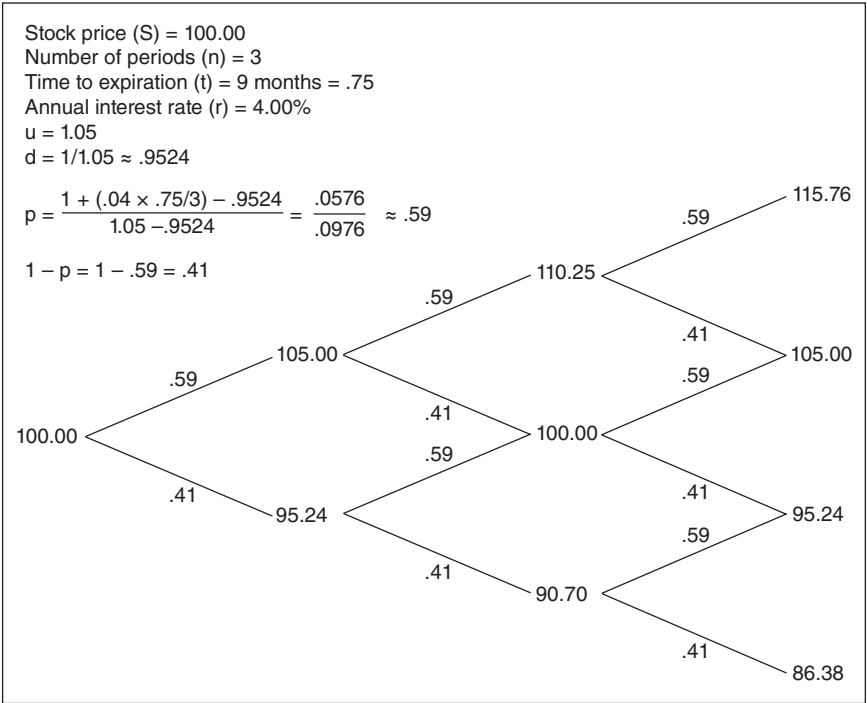
Figure 19-1 A three-period binomial tree.
