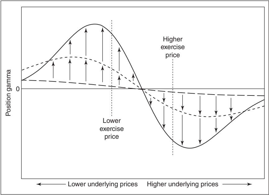
Figure 12-10 Gamma of a bull spread as time passes or volatility declines.
