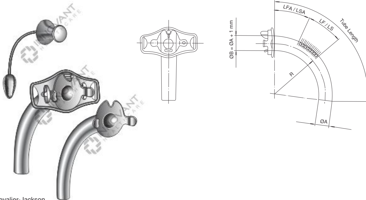
Chevalier-Jackson Outer Tube Sieve Inner Tube Sieve
