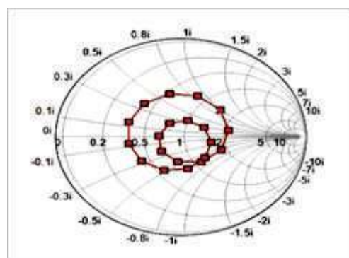
Smith Chart
