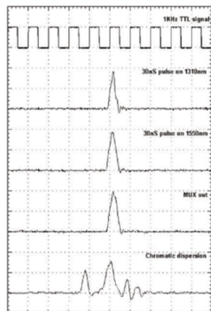
Chromatic Dispersion Using FOL-DUAL/ FOL-PASSIVE/ FOL-CD
