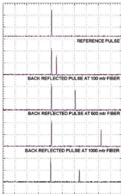
Principle of OTDR Using FOL-DUAL/ FOL-PASSIVE/ FOL-FIBER
