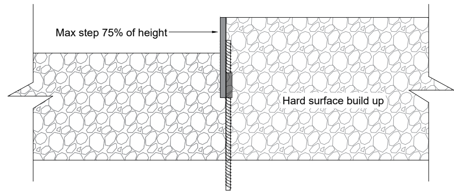
Detail 3 Hard Landscape/Hard Landscape(no concrete)
