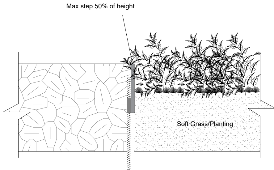
Detail 1 Soft Landscape/Soft Landscape(no concrete)
