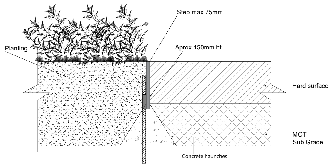
Detail 2 Kerb detail install(haunch)
