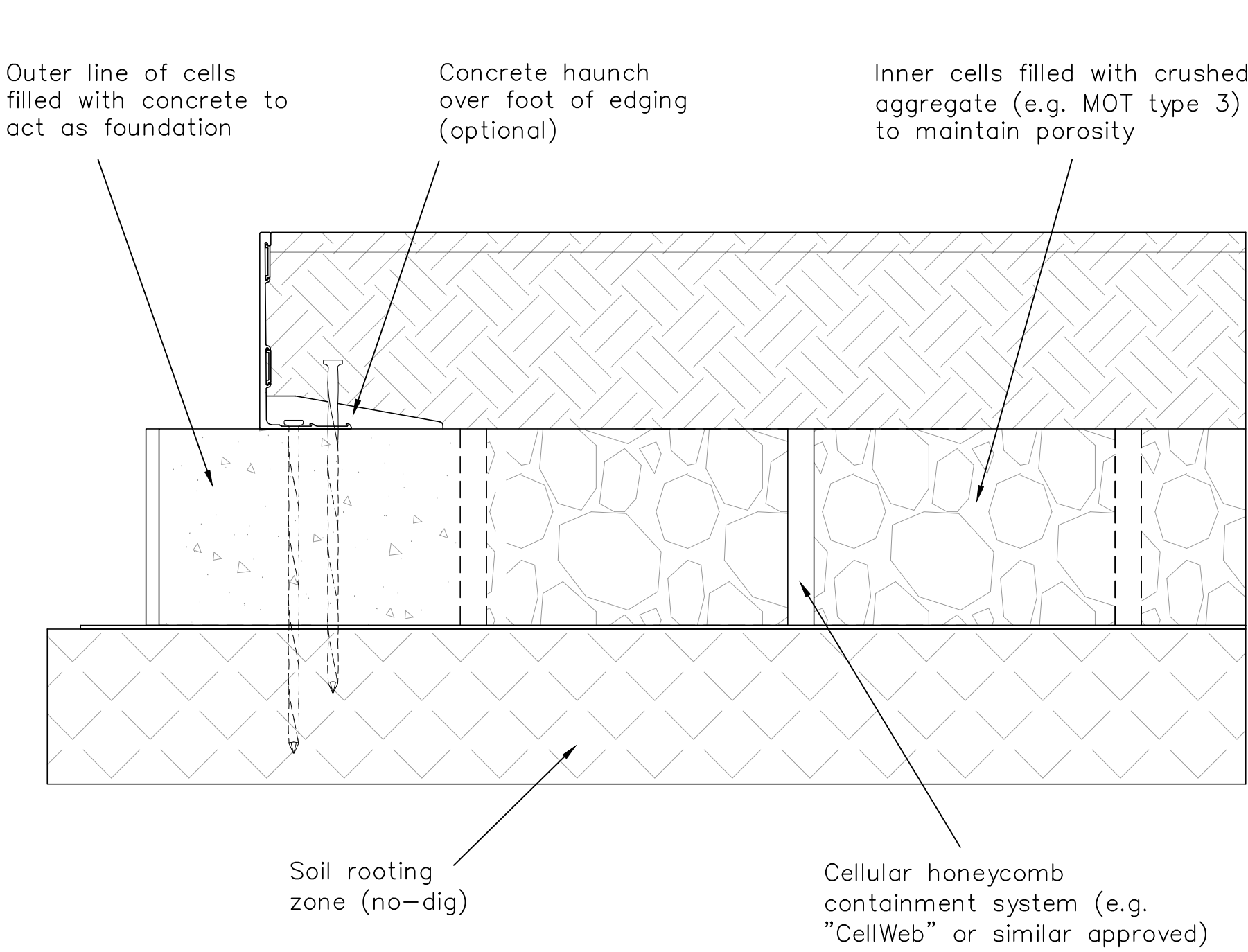
Detail 3 No-Dig
