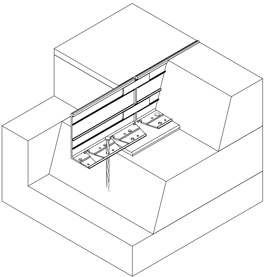
ISOMETRIC CUT-AWAY VIEW NTS
