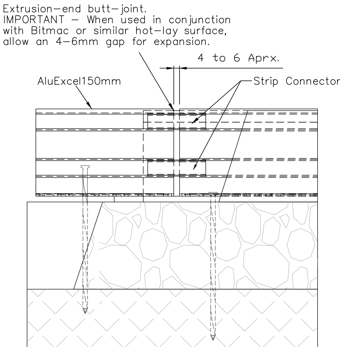
JOINER DETAIL SCALE 1:4
