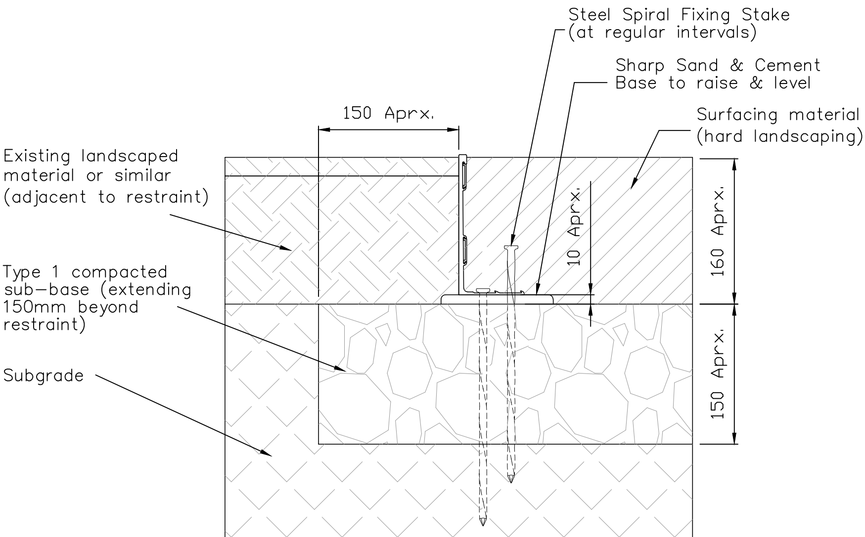
SECTION SCALE 1:4
