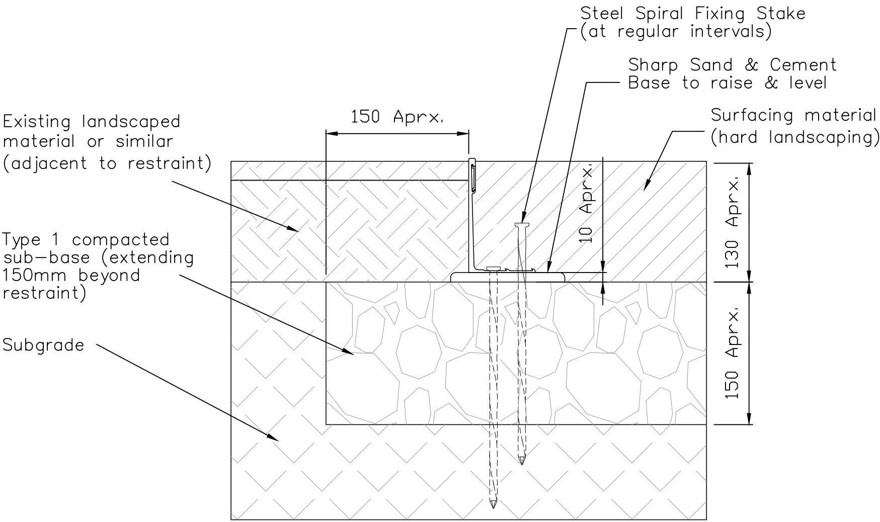
SECTION SCALE 1:4
