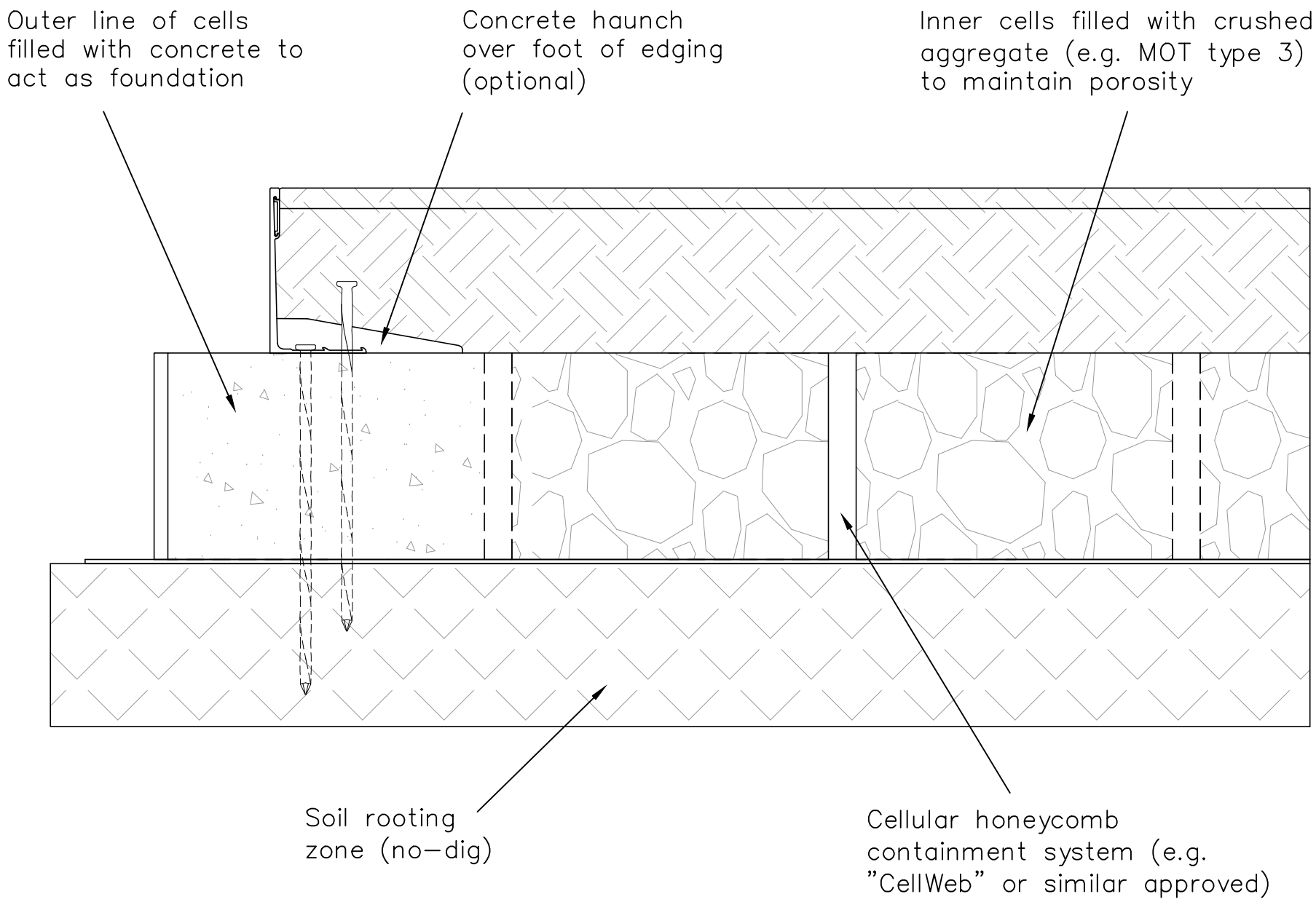
Detail 3 No-Dig
