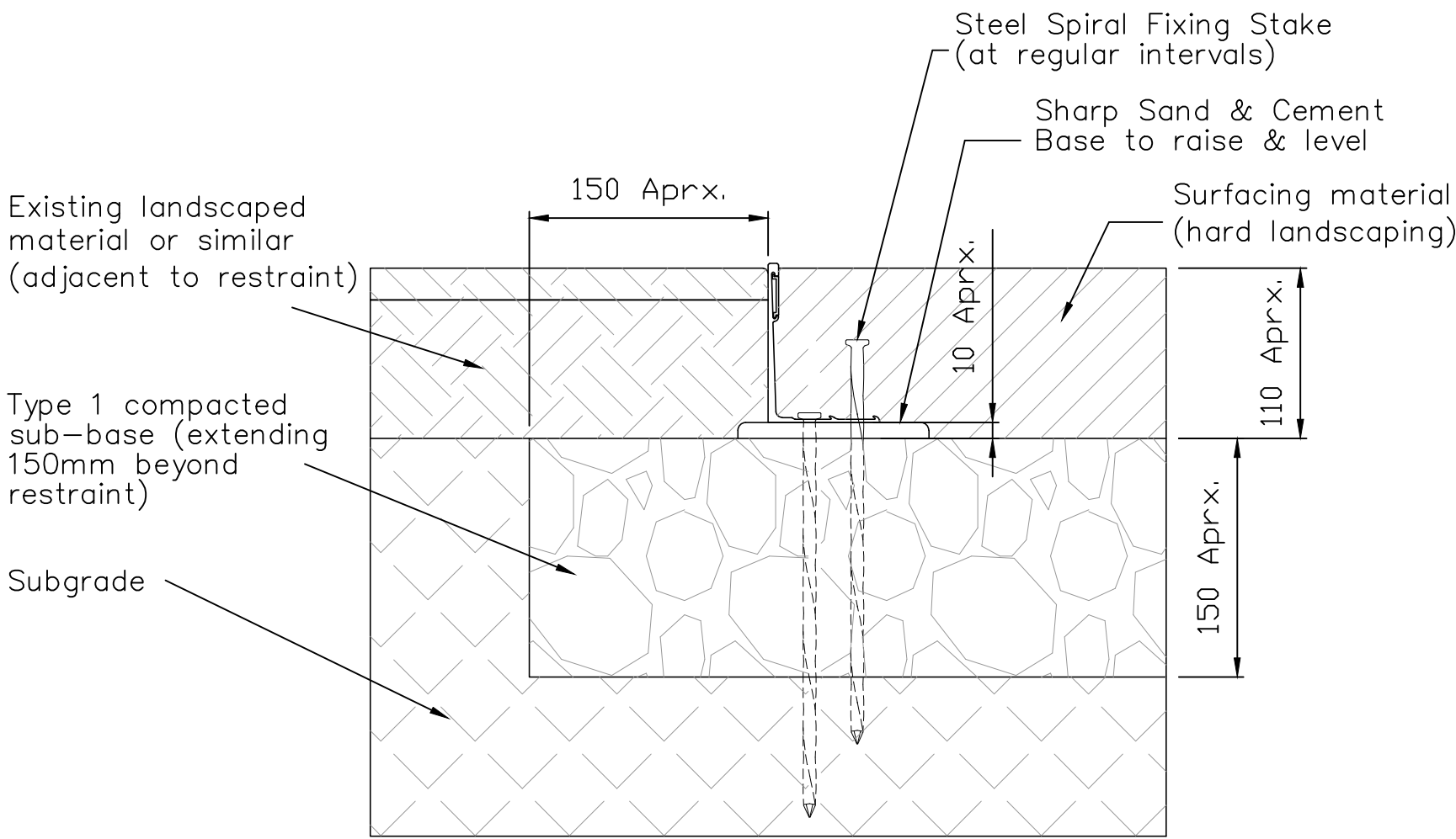
SECTION SCALE 1:4
