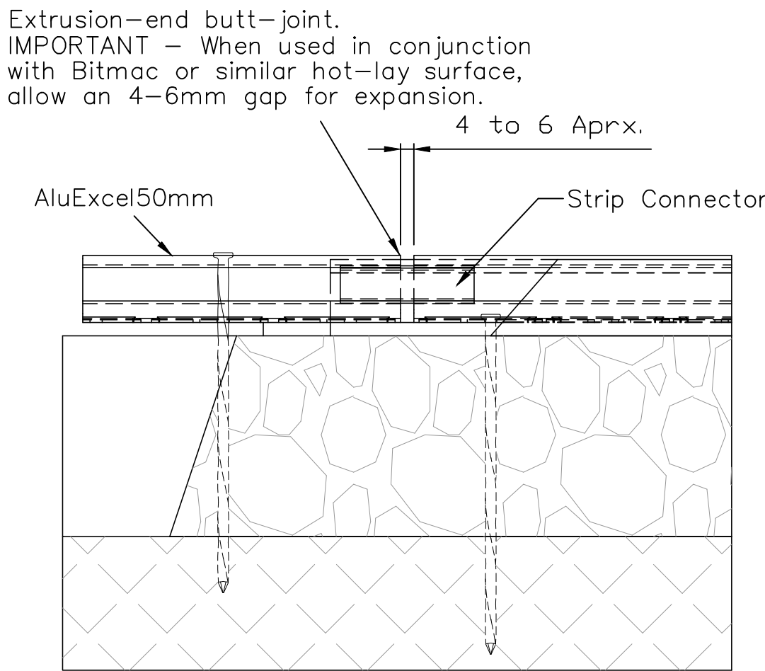
JOINER DETAIL SCALE 1:4
