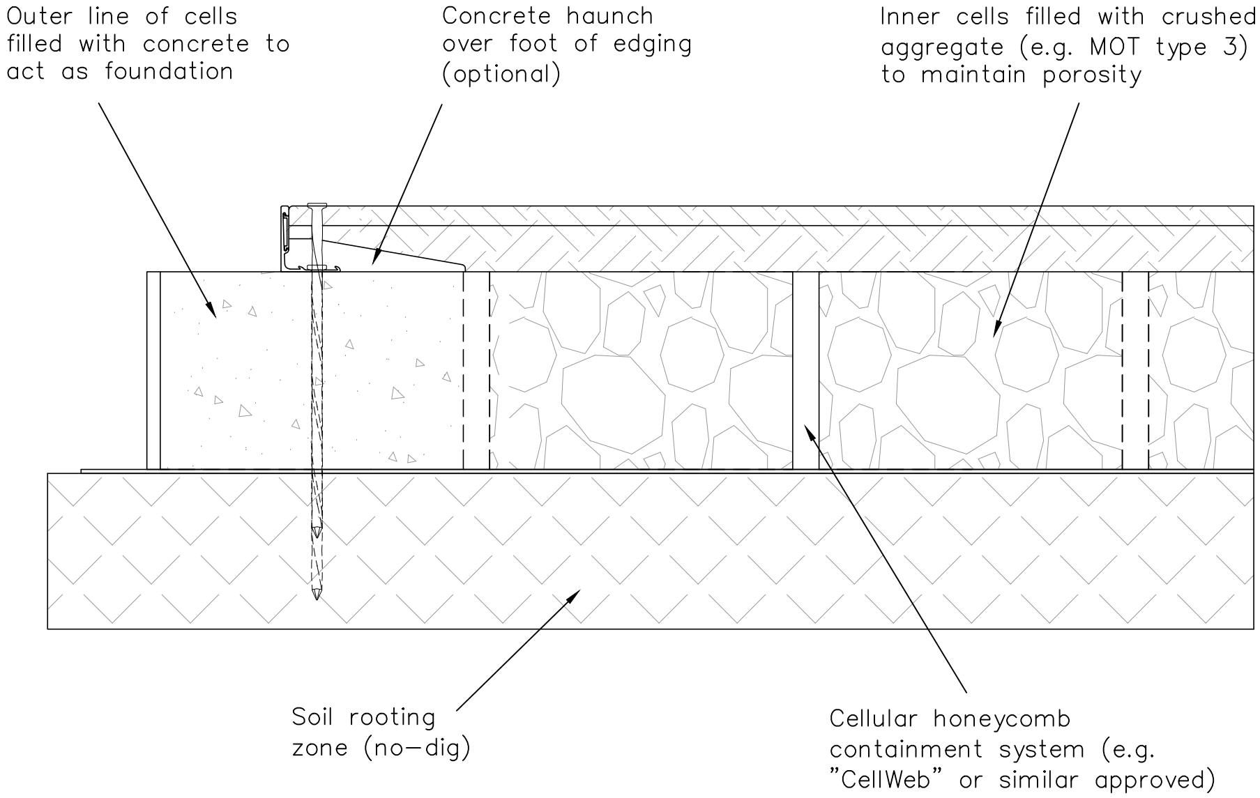
Detail 3 No-Dig
