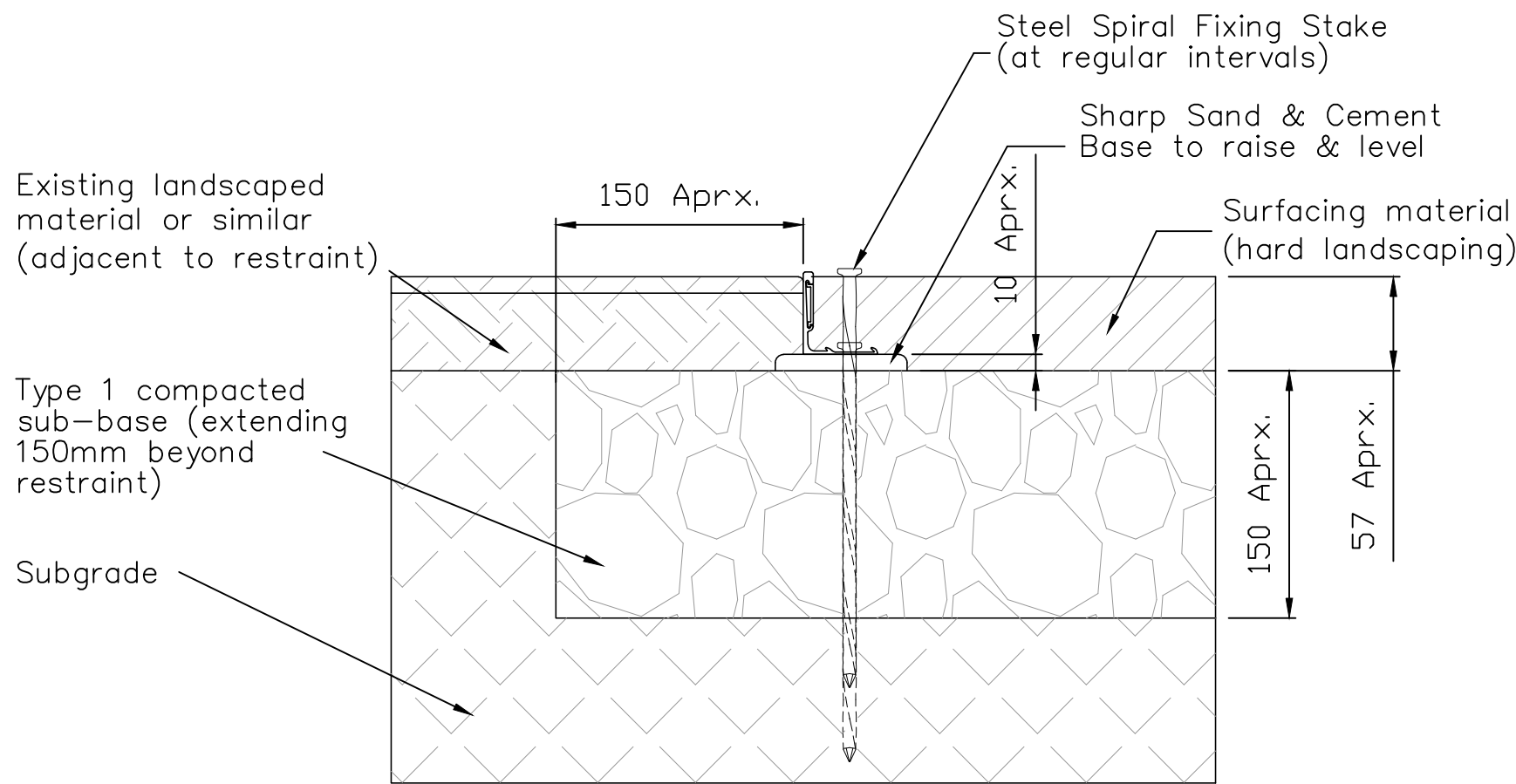
SECTION SCALE 1:4
