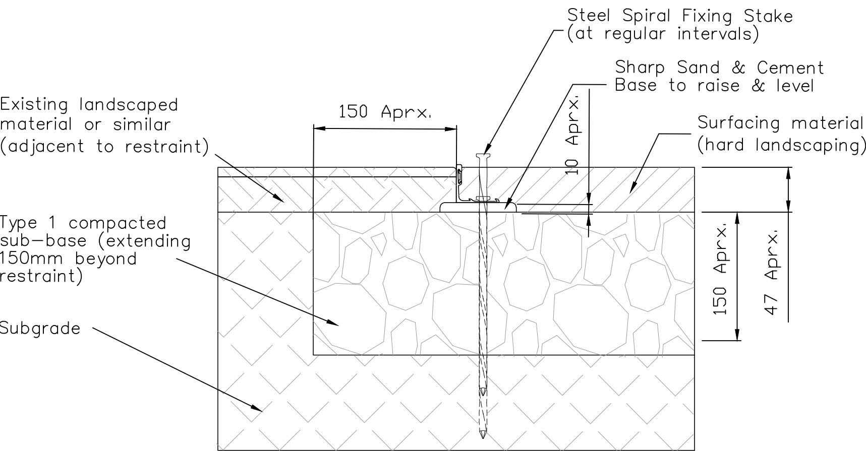
SECTION SCALE 1: 4
