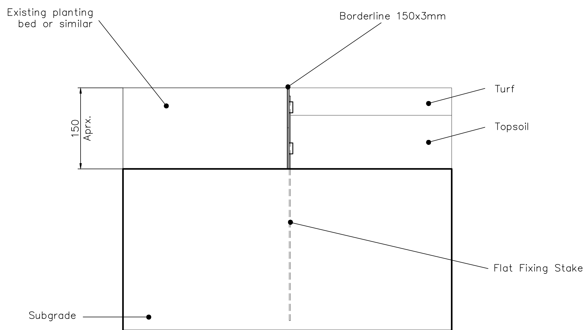
SECTION SCALE 1:4
