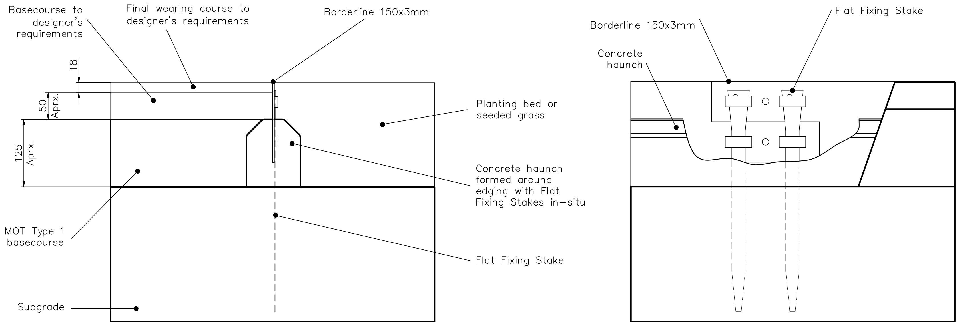
SECTION SCALE 1:4
