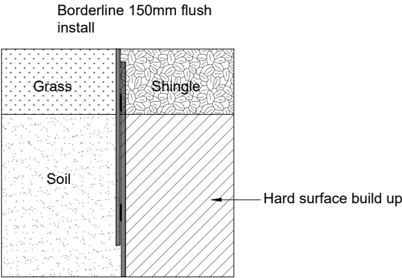
Detail 2 Soft/hard
