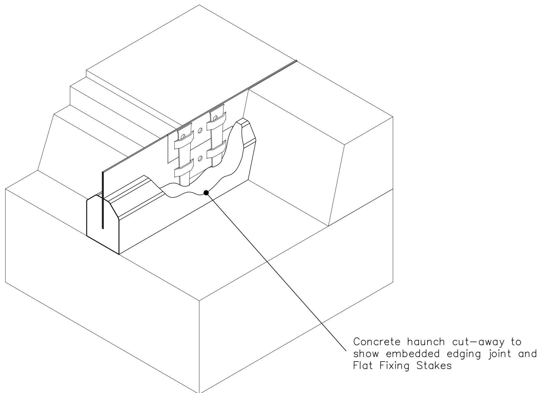
ISOMETRIC CUT-AWAY VIEW NTS
