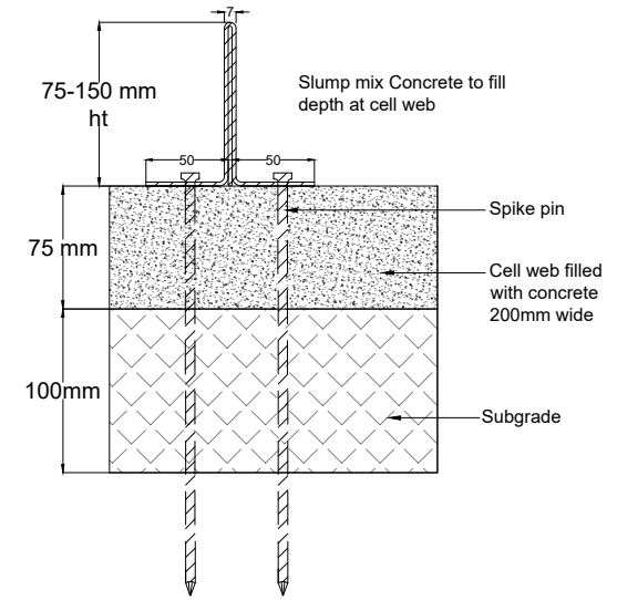
Detail 3 Minimum dig/cell web install
