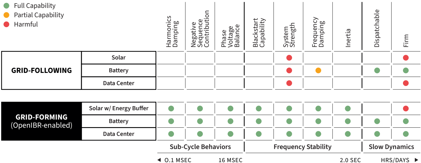
FIGURE 2 Power Electronics Providing Stability & Resilience
