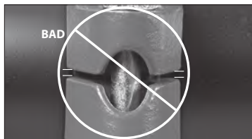
IMPROPERLY ASSEMBLED JOINT – BOLT PAD GAP/UNDER-TIGHTENED
