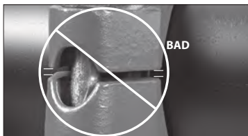
IMPROPERLY ASSEMBLED JOINT – BOLT PAD GAP/UNDER-TIGHTENED
