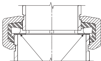
Assembly Washer
