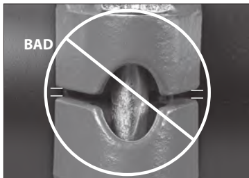
IMPROPERLY ASSEMBLED JOINT – BOLT PAD GAP/UNDER-TIGHTENED
