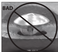
OVAL NECK OF BOLT NOT SEATED PROPERLY
