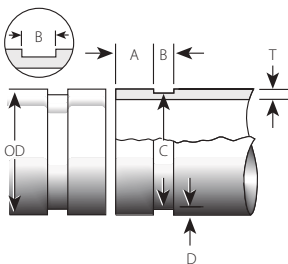
Cut Groove
