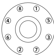
8-Bolt Tightening Pattern
