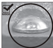
OVAL NECK OF BOLT SEATED PROPERLY
