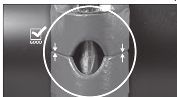
PROPERLY ASSEMBLED JOINT – METAL-TO-METAL CONTACT AS INDICATED
