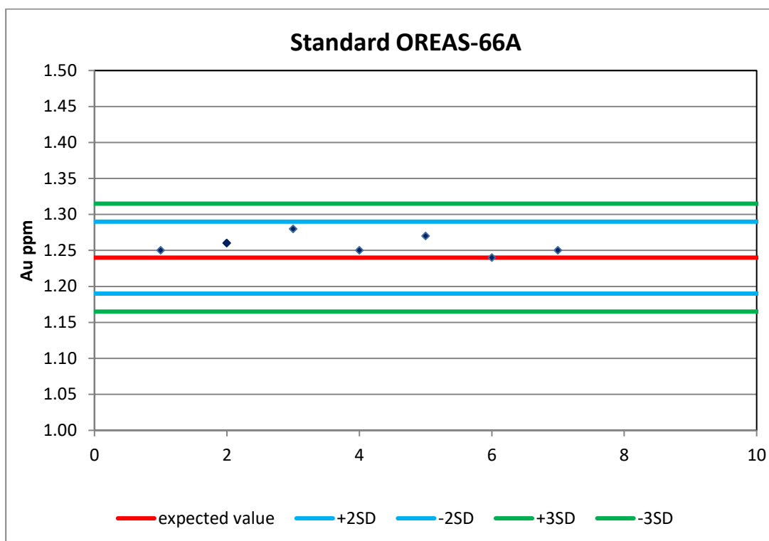
Figure 11.8 Analyses of Standard OREAS-66A
