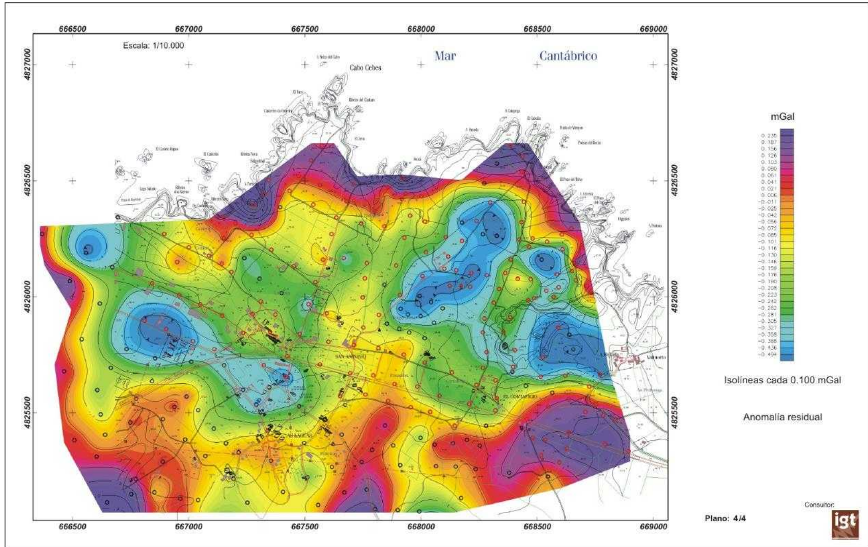
Figure 6.2 Residual Gravity of the Salave Area (From Valdés Suárez, 2012)
