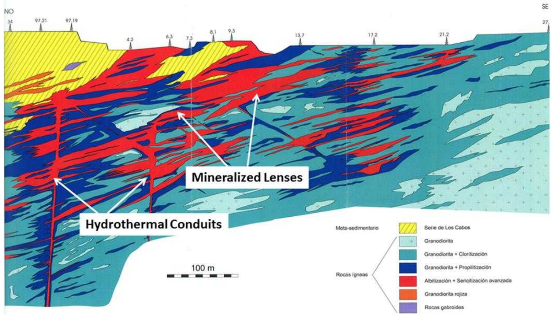
Figure 7.5 Schematic NW-SE Cross Section of Alteration at Salave Showing Relationship to Mineralization (modified from Rodriguez Terente, 2007; NW/SE cross section)
