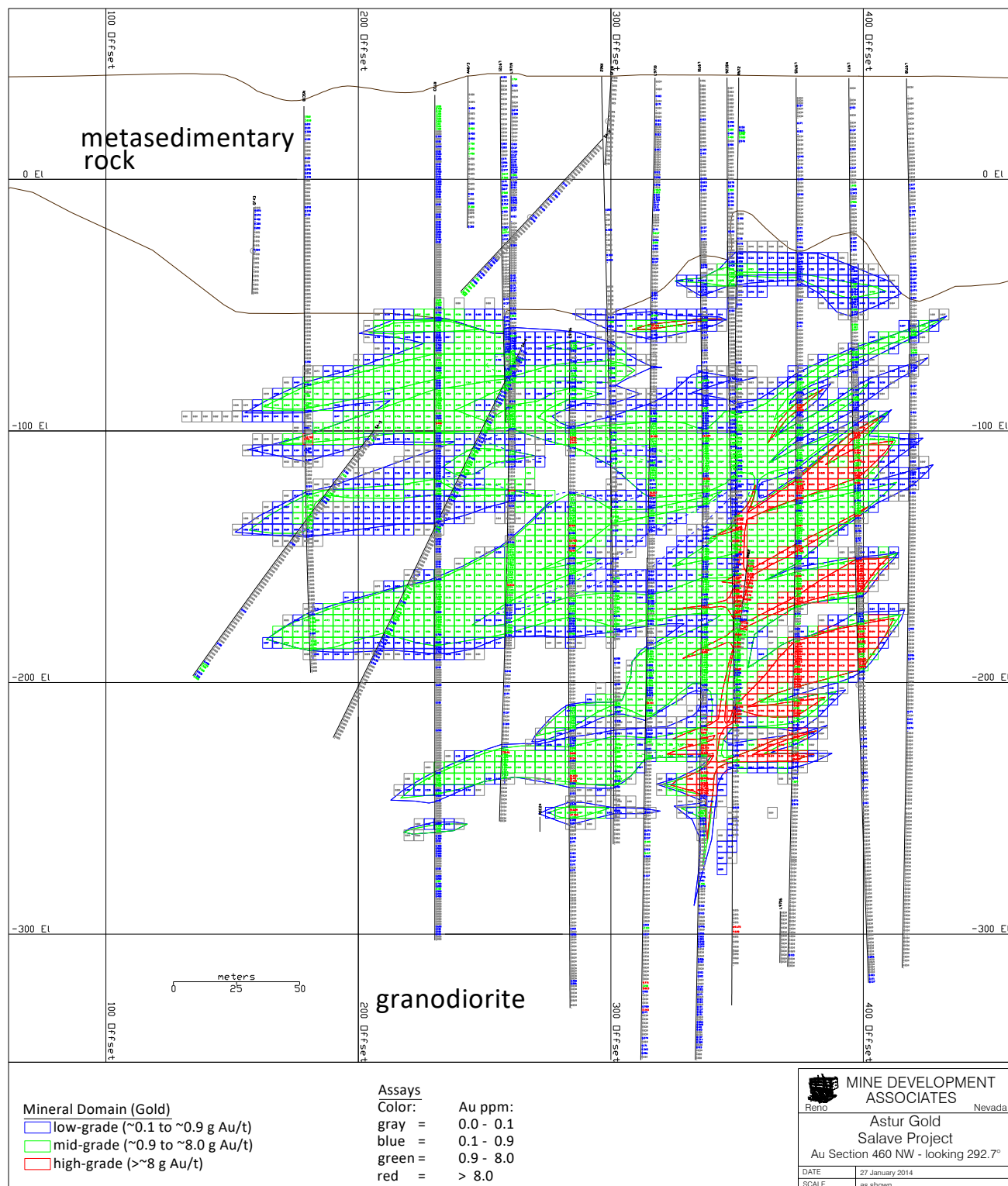
Figure 14.4 Salave Deposit Cross Section 460NW Showing Block Model Gold Grades
