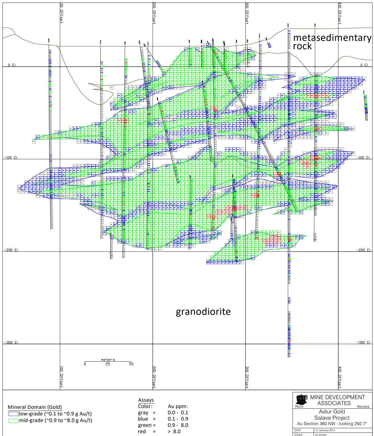
Figure 14.3 Salave Deposit Cross Section 360NW Showing Block Model Gold Grades
