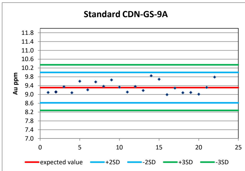
Figure 11.5 Analyses of Standard CDN-GS-9A
