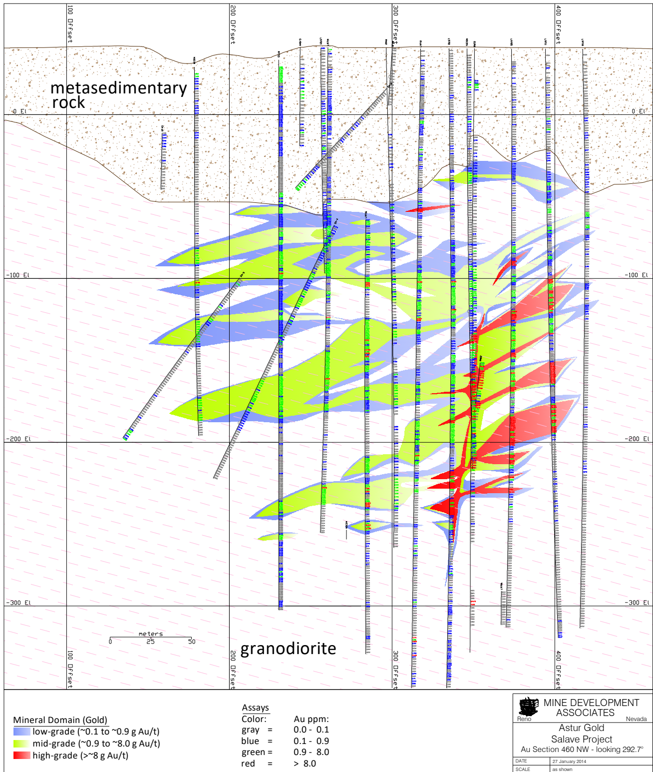
Figure 14.2 Salave Deposit Cross Section 460NW Showing Gold Mineral Domains
