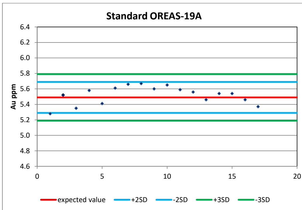
Figure 11.6 Analyses of Standard OREAS-19A
