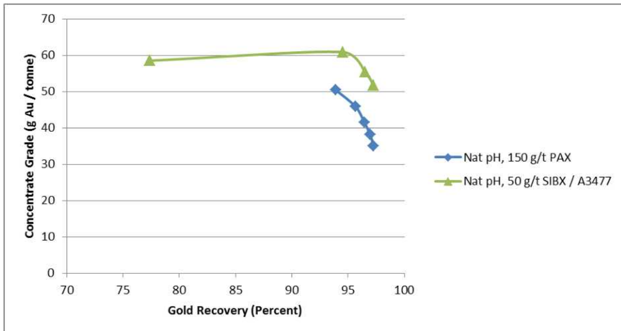
Figure 13.2 AMMTEC Upper Zone Grade-Recovery Curve
