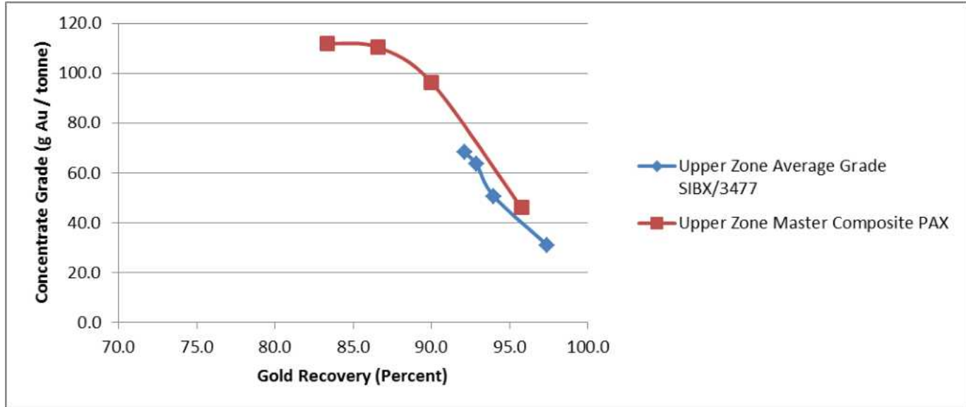
Figure 13.3 ALS-Met Upper Zone Grade-Recovery Curve
