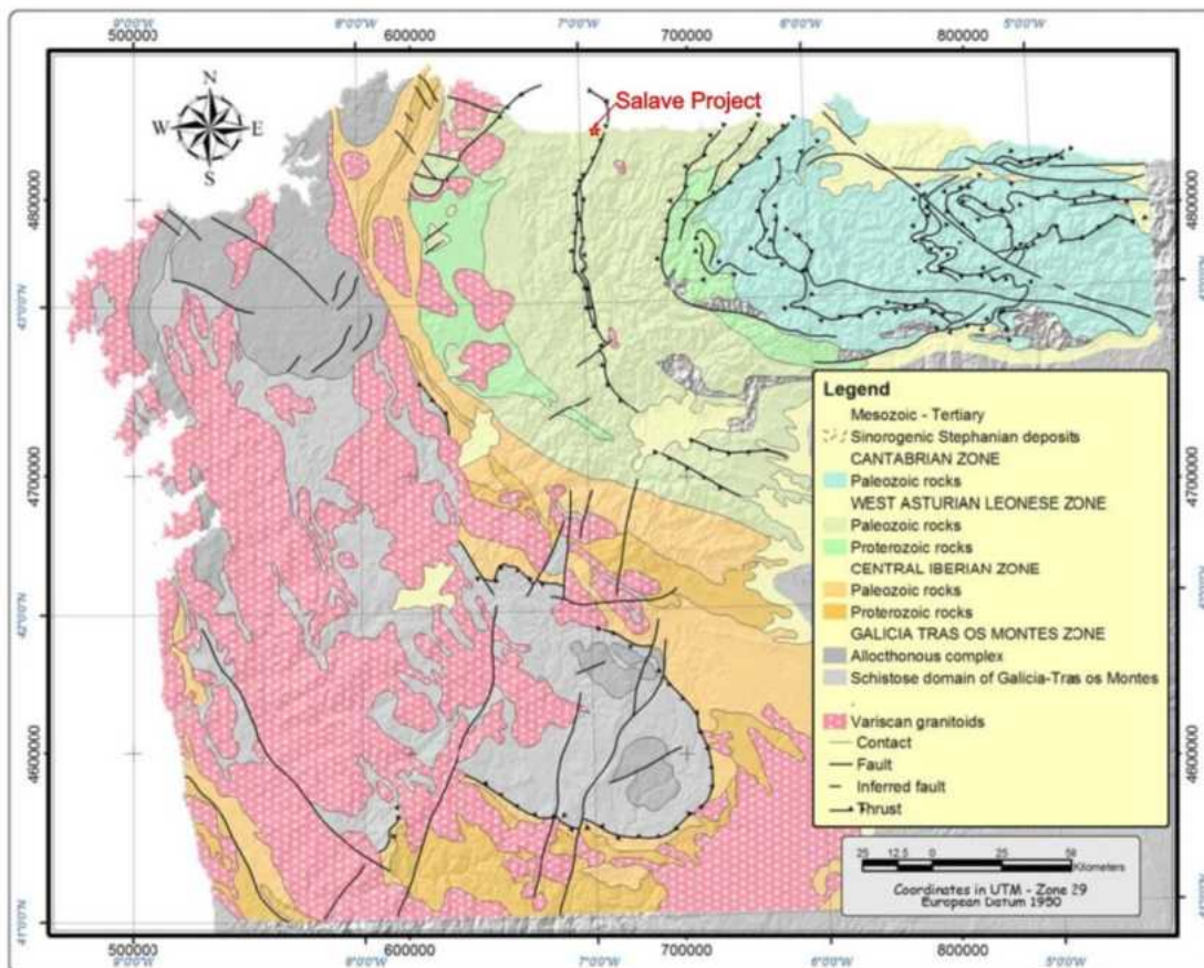
Figure 7.1 Geologic Map of the Northwestern Part of the Iberian Peninsula (from Nieto, 2004)
