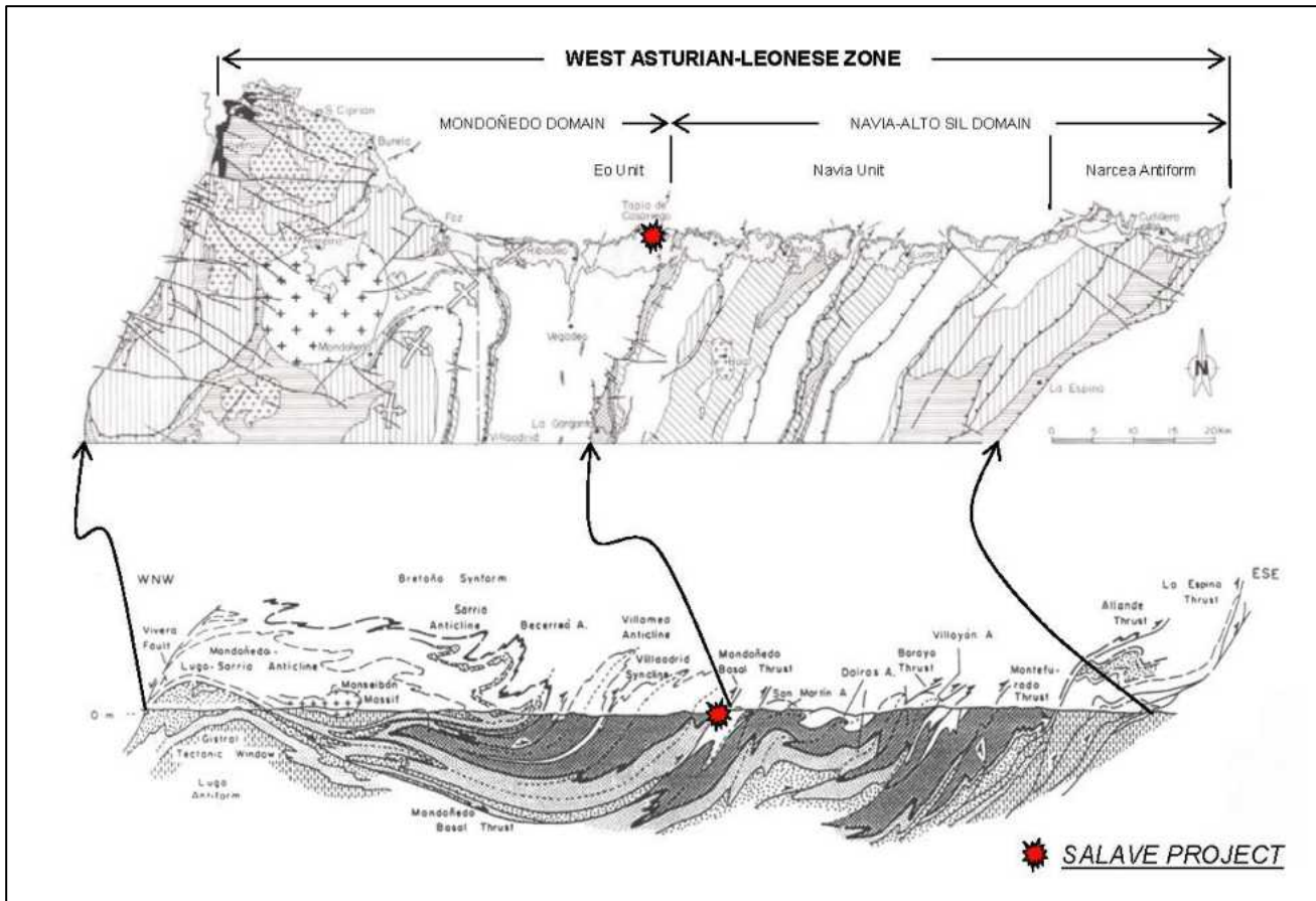
Figure 7.2 Deformation in the West Asturian–Leonese Zone (from Nieto, 2004)
