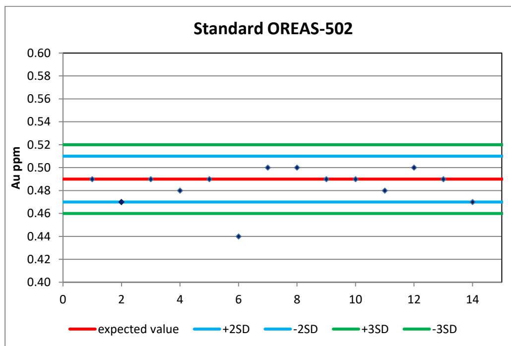
Figure 11.7 Analyses of Standard OREAS-502
