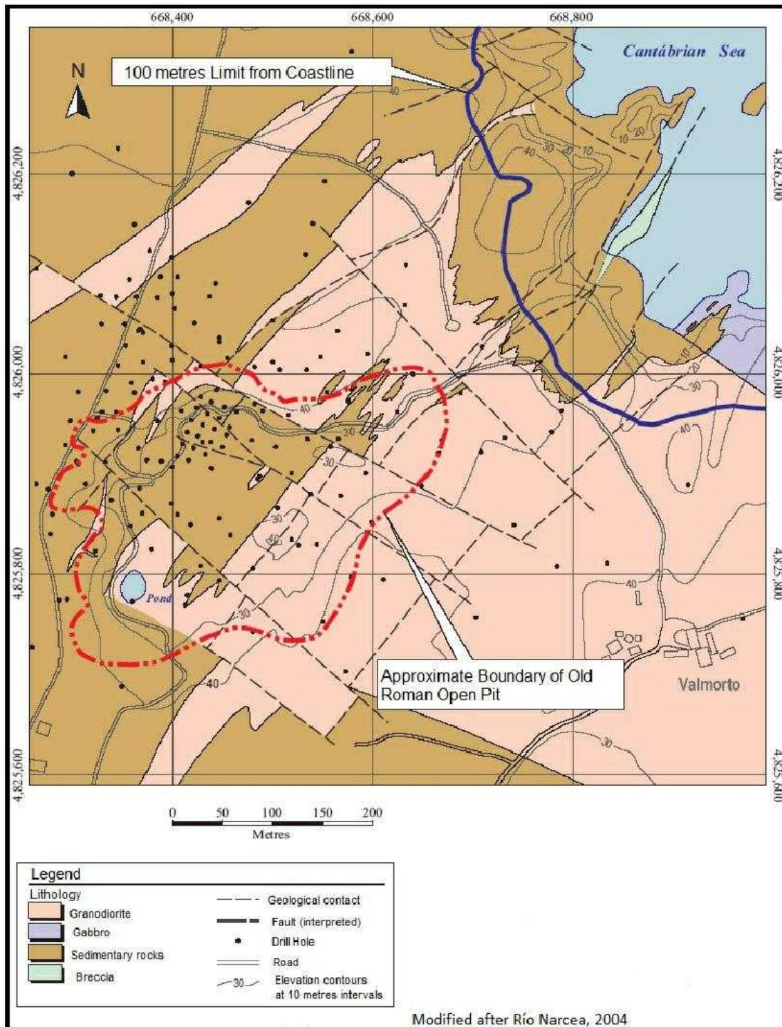
Figure 7.4 Property Geology at the Salave Project (from Tenorio, 2011, based on information from Rio Narcea Mines Ltd.)
