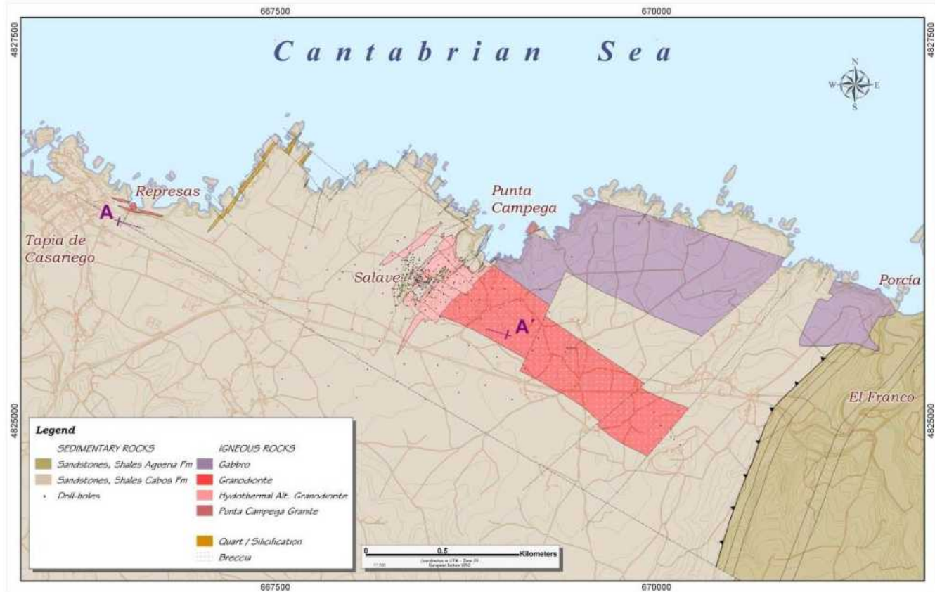
Figure 7.3 Local Geology of the Salave Gold Project (from Nieto, 2004)
