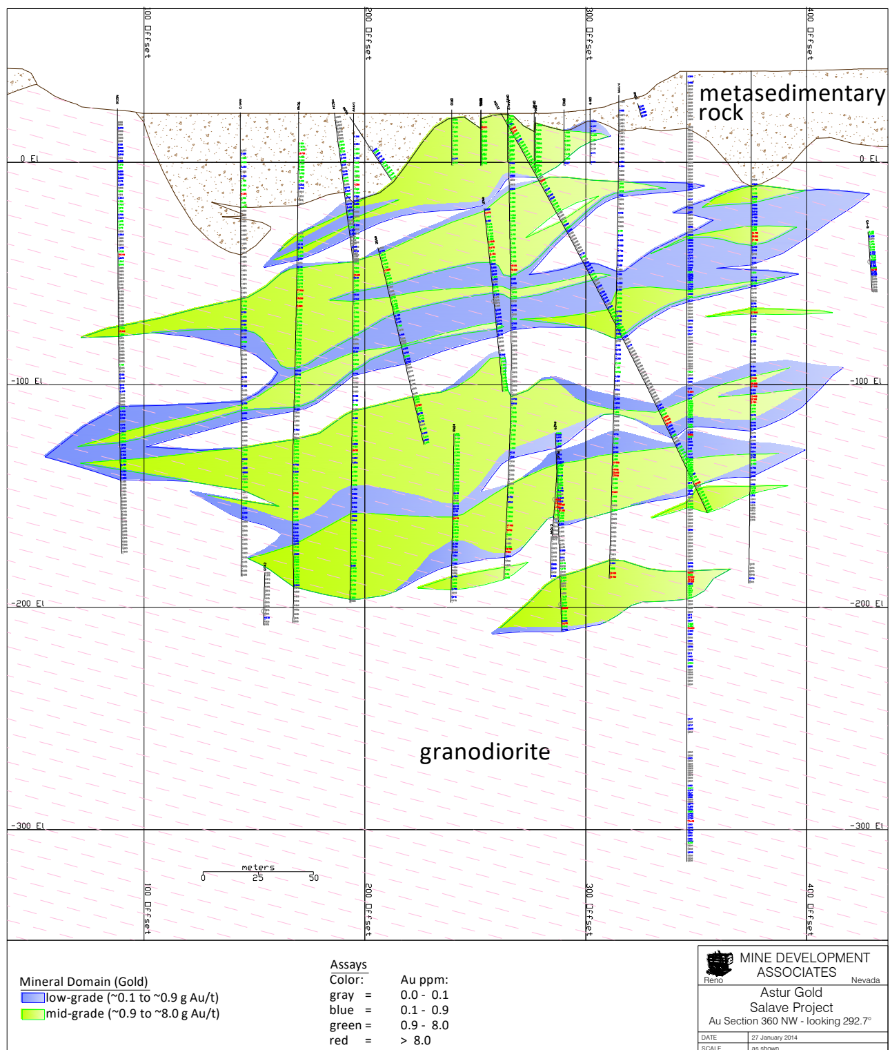
Figure 14.1 Salave Deposit Cross Section 360NW Showing Gold Mineral Domains
