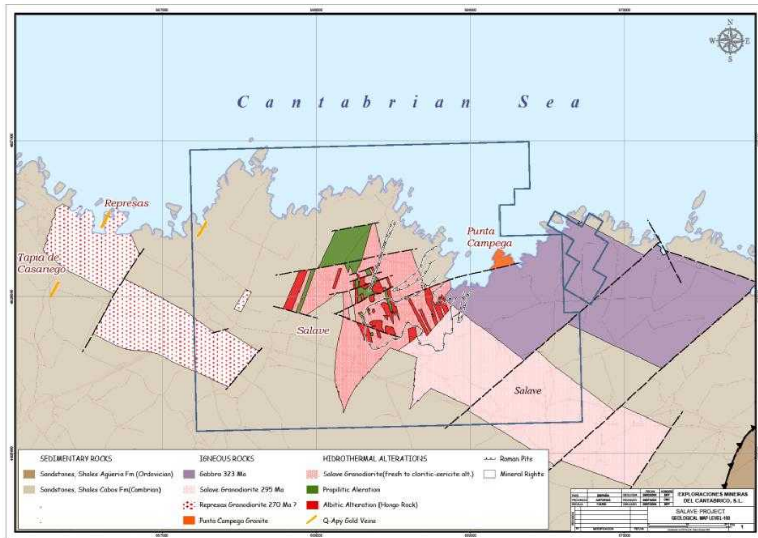
Figure 7.6 Plan Map of Geology and Alteration of the Salave Area (Provided by Astur)
