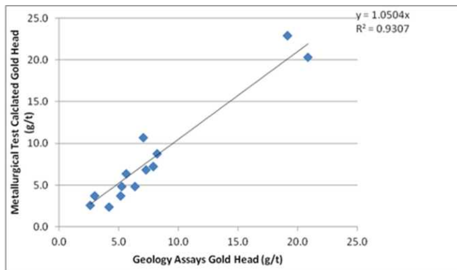
Figure 13.1 Metallurgical Calculated Gold Head vs. Geologic Calculated Gold Head
