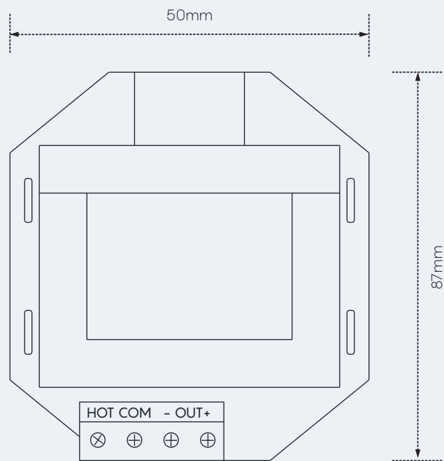
Rear Dimension
