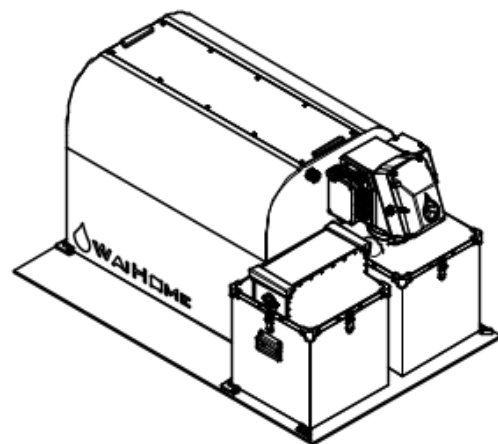
Isometric View SCALE 1:32
