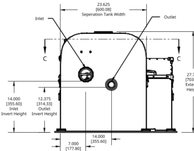
End View
