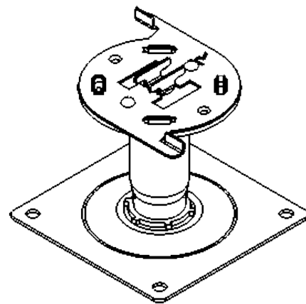
Preventa Steel Fire - Resistant Adjustable Pedestal 90 - 140mm External Zintek Finish Part Code: 341015
