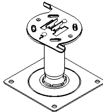
Preventa Steel Fire - Resistant Adjustable Pedestal 110 - 185mm External Zintek Finish Part Code: 341016
