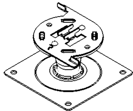
Preventa Steel Fire - Resistant Adjustable Pedestal 60 - 90mm External Zintek Finish Part Code: 341014
