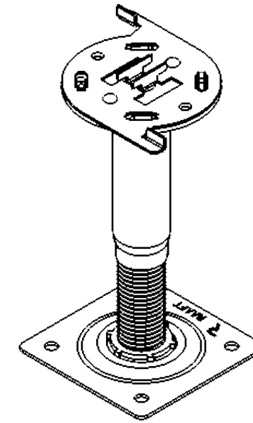
Preventa Steel Fire - Resistant Adjustable Pedestal 110 - 185mm External Zintek Finish Part Code: 341017
