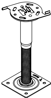
Preventa Steel Fire - Resistant Adjustable Pedestal 250 - 325mm External Zintek Finish Part Code: 341018
