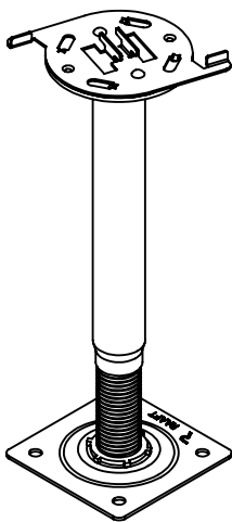
Preventa Steel Fire - Resistant Adjustable Pedestal 300 - 375mm External Zintek Finish Part Code: 341019
