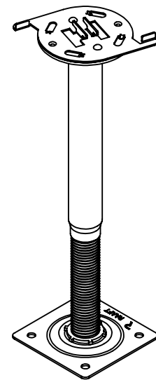
Preventa Steel Fire - Resistant Adjustable Pedestal 350 - 425mm External Zintek Finish Part Code: 341020
