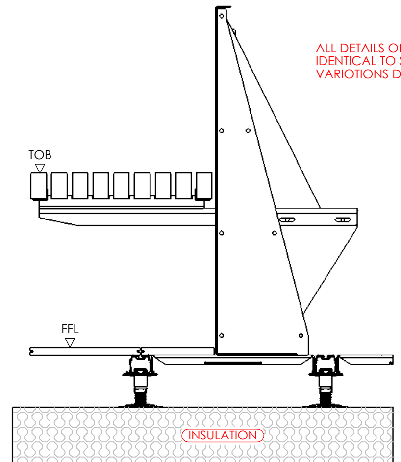
PLANTERLINE STRAIGHT - LONG SLAT CANTILEVER BENCH SITUATED ON RAAFT FLOOR STRUCTURE PANELS
