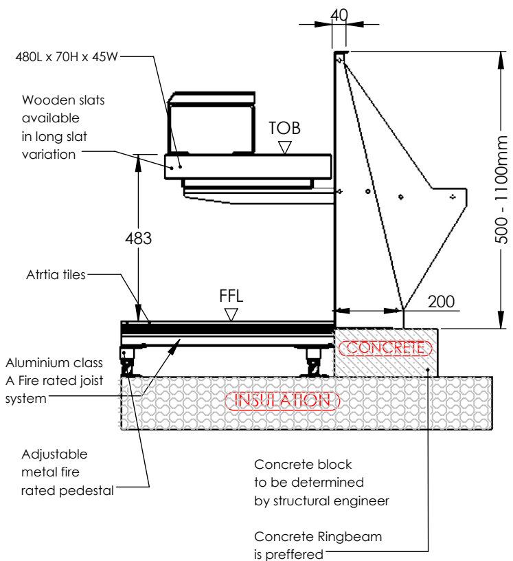
PLANTERLINE STRAIGHT - CANTILEVER BENCH SITUATED ON CONCRETE
