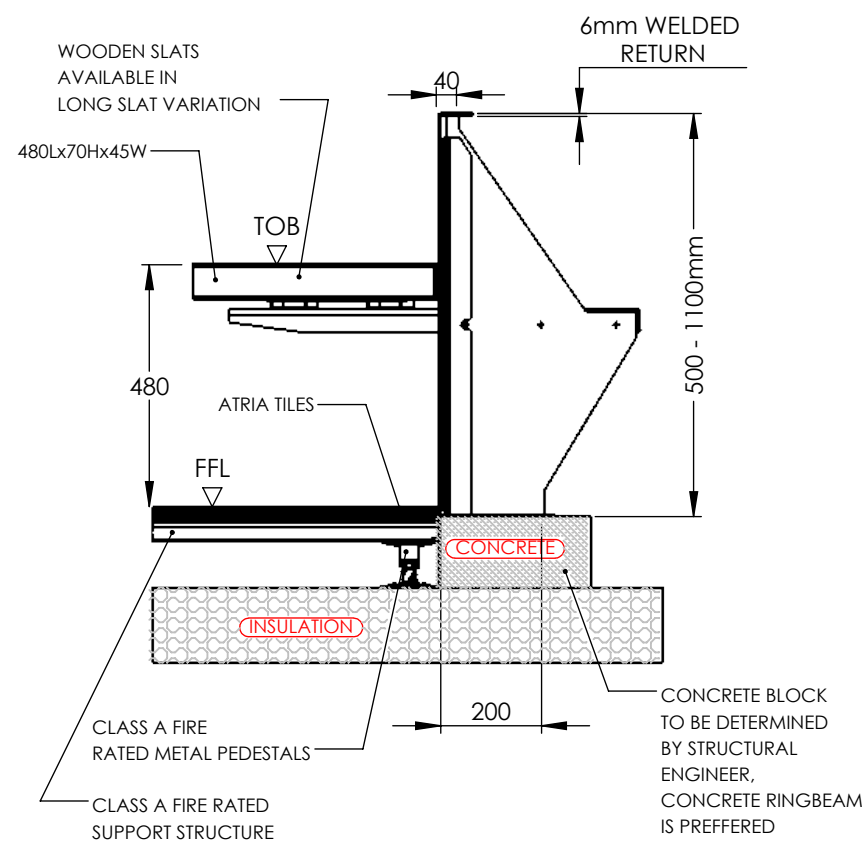
PLANTERLINE CURVE - CANTILEVER BENCH SITUATED ON CONCRETE
