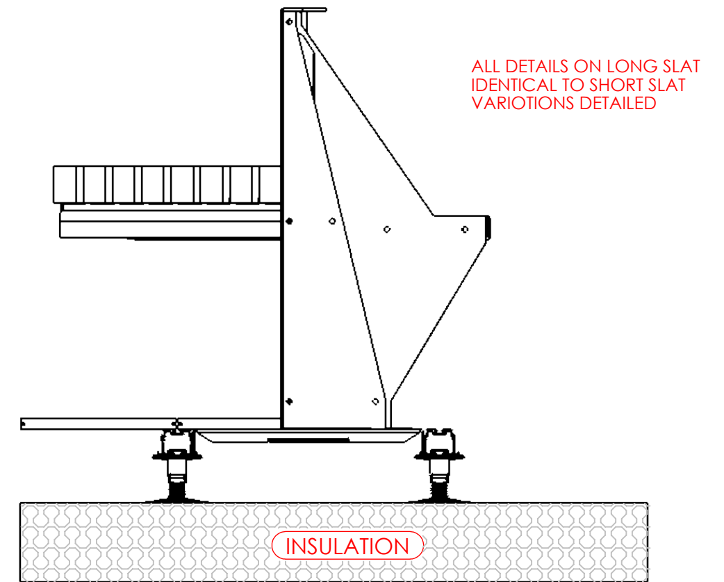
PLANTERLINE CURVE - CANTILEVERED LONG SLAT BENCH SITUATED ON FLOOR STRUCTURE PANELS
