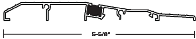
ADA Outswing Sill
