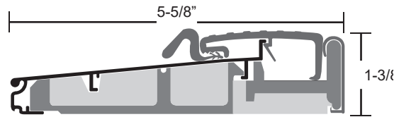
Bumper Outswing Sill
