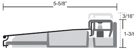
Adjustable Inswing Z Sill (standard)
