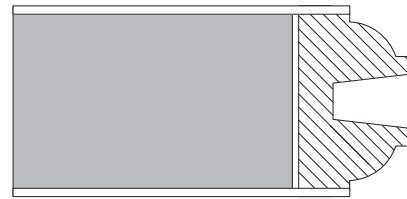
Woodgrain Ovolo Sticking Profile
