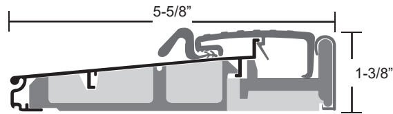
Bumper Outswing Sill
