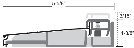
Adjustable Inswing Z Sill (standard)
