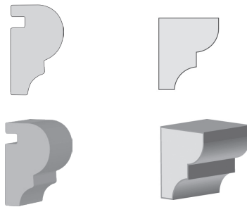
8081 Nosing/Cove 8181 Super Cove 1-1/8" x 1-13/16" 5/8" x 3/4"
