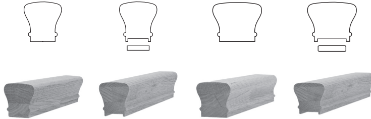
6010 Rail 2-1/4" x 2-3/8" 6010P Rail 2-1/4" x 2-3/8" 1-1/4" Plow Includes 6107 fillet 6210 Rail 2-5/8" x 2-3/8" 6210P1 Rail 2-5/8" x 2-3/8" 1-3/4" Plow Includes 6007 fillet
