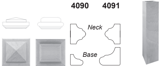
Pyramid & Square Replacement Cap Set
