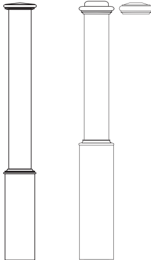
4093 Plain Panel 4-3/4" Post 6-1/4" Base 4097 Plain 6" Post 7-1/2" Base
