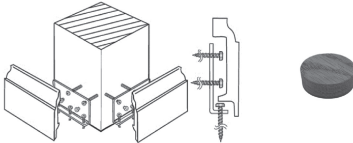
3007_ For 3" Newels 3008_ For 3-1/2" Newels 3000_ 1" Flat Plug Face Grain
