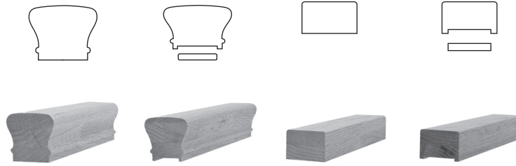
6210 Rail 2-5/8" x 2-3/8" 6210P1 Rail 2-5/8" x 2-3/8" 1-3/4" Plow Includes 6007 fillet 6770* Rail 2-1/4" x 1-9/16" 6770P1* Rail 2-1/4" x 1-9/16" 1-3/4" plow Includes 6007 fillet
