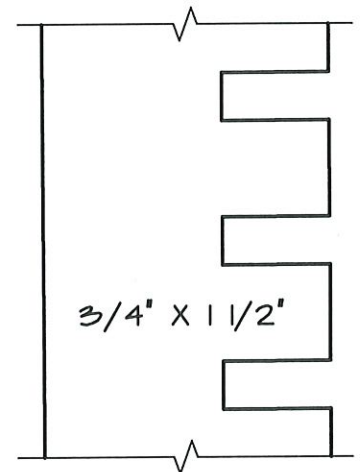
DENTIL MOULD
