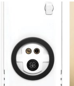
The underside of the GT 1230, with integrated cargo sensor and tamper detection seal.
