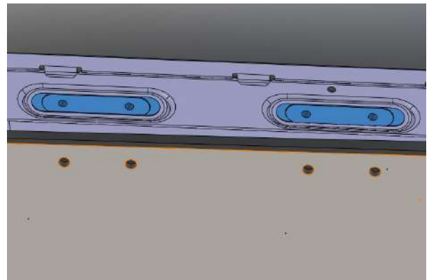
▲ Figure 32. Correct alignment of the Pill Box Bracket and pill shaped holes. (top brackets hidden to show alignment)
