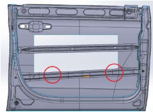
▲ Figure 21. Crash bar bracket location
