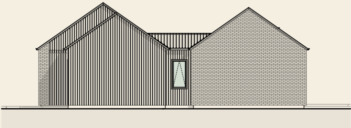
South Elevation Scale 1:120
