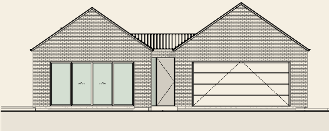
North Elevation Scale 1:120
