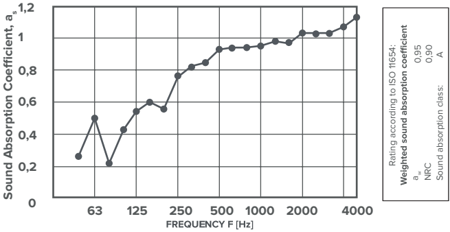
Plate 12mm Natural + Fetfill (100cm Air Gap)
