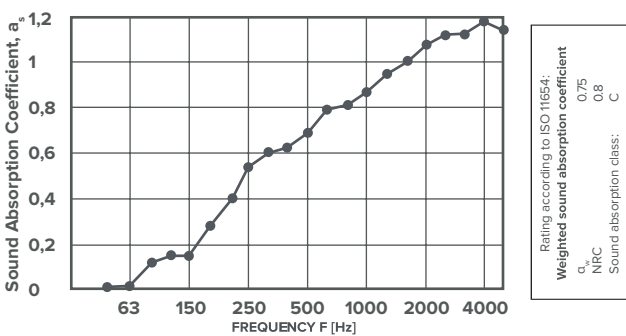
Plate 12mm Natural (50cm Air gap, 10cm Axis)
