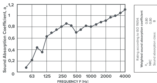
Plate 12mm Natural (40cm Air Gap)
