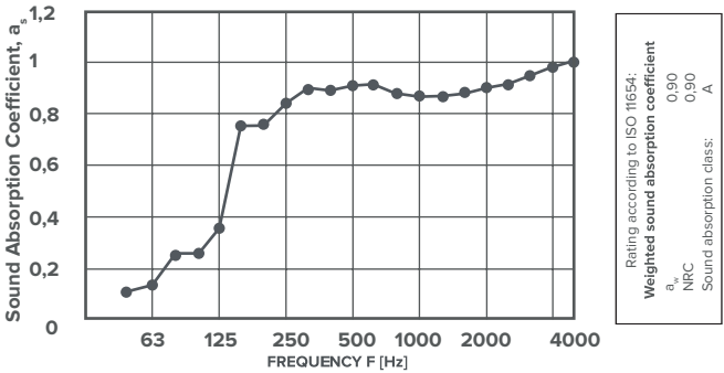
Plate 12mm Mandarin + Fetfill (30cm Air Gap)
