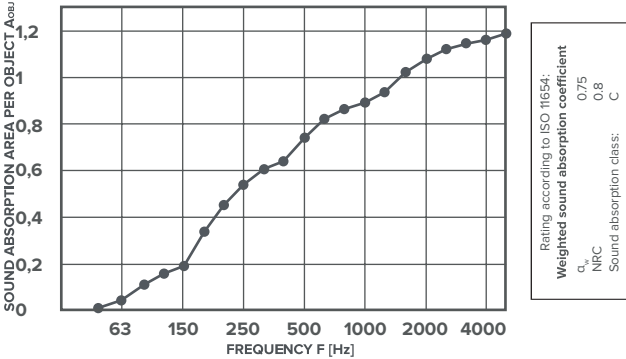
Plate 12mm Mandarin (50cm Canopy, 10cm Axis)
