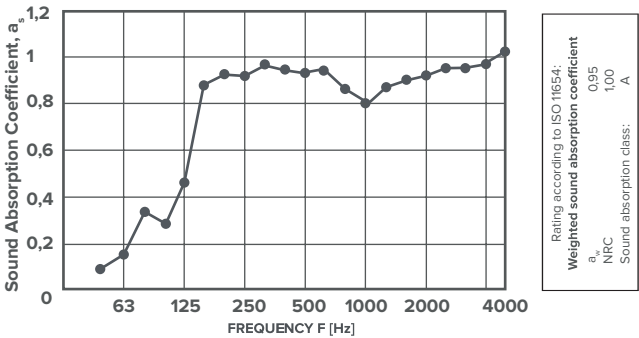
Plate 12mm Mandarin + Fetfill (40cm Air Gap)
