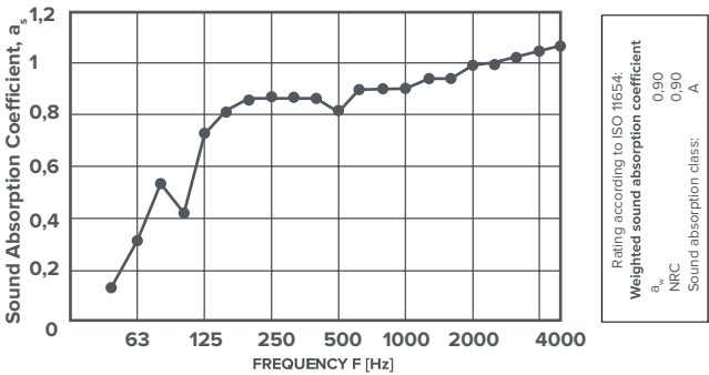
Plate 12mm Natural + Fetfill (40cm Air Gap)
