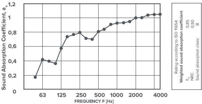
Plate 12mm Mandarin + Fetfill (50cm Air Gap)
