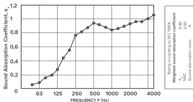
Plate 12mm Natural (20cm Air Gap)
