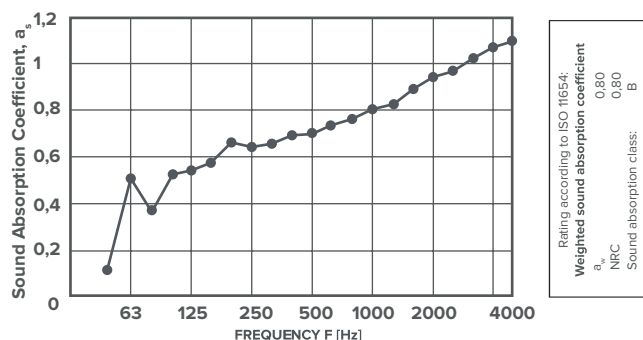
Plate 12mm Mandarin (70cm Air Gap)
