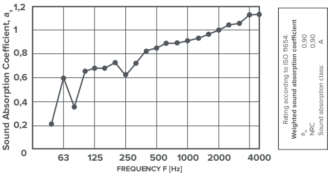
Plate 12mm Mandarin + Fetfill (70cm Air Gap)
