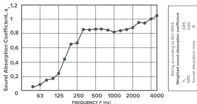
Plate 12mm Mandarin (20cm Air Gap)
