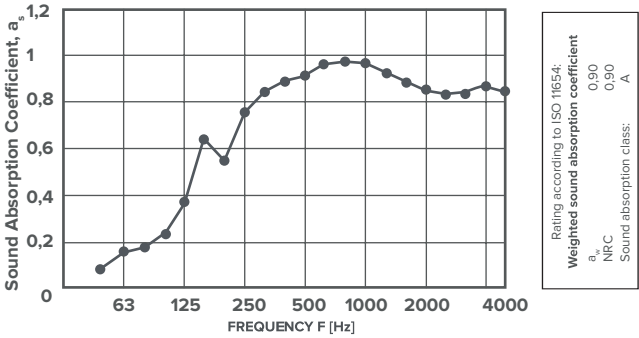
Plate 12mm Natural + Fetfill (20cm Air Gap)
