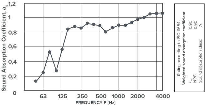
Plate 12mm Natural + Fetfill (50cm Air Gap)
