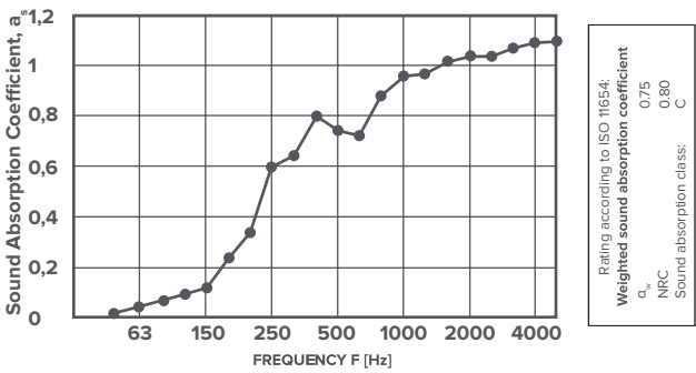
Plate 12mm Natural (30cm Air Gap, Canopy)
