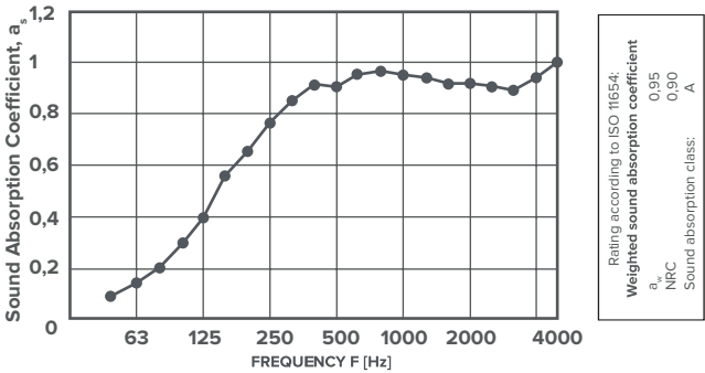
Plate 12mm Mandarin + Fetfill (20cm Air Gap)
