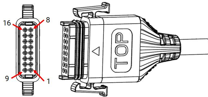
Figure 9: GT 12xx Cable Assembly
