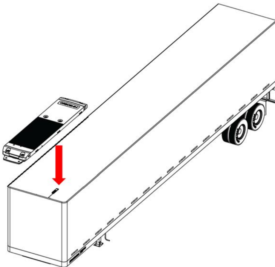
Figure 3: Front Mounting Location on the Roof of a Trailer
