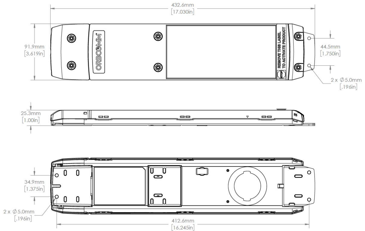
Figure 5: GT 12xx with Connector
