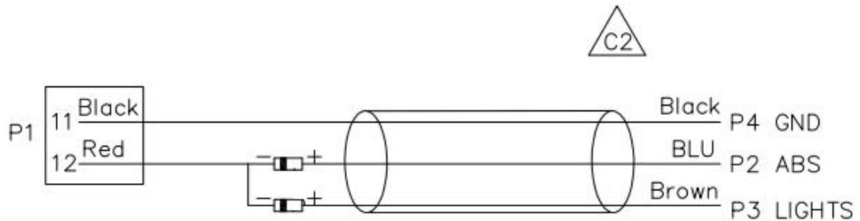
Figure 11: Circuit Diagram
