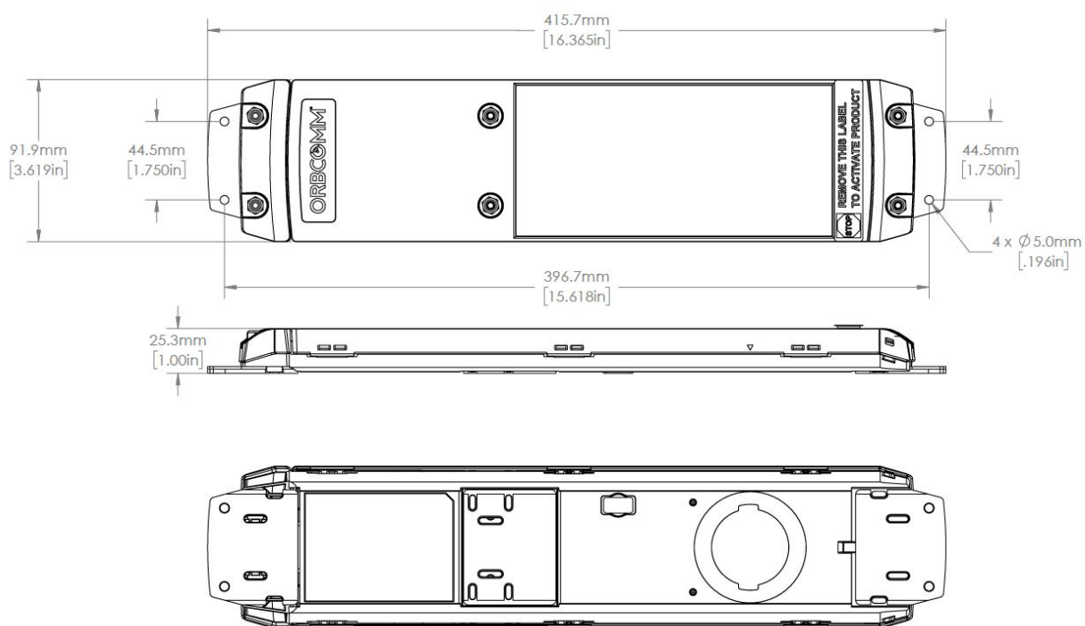
Figure 6: GT 12xx without Connector
