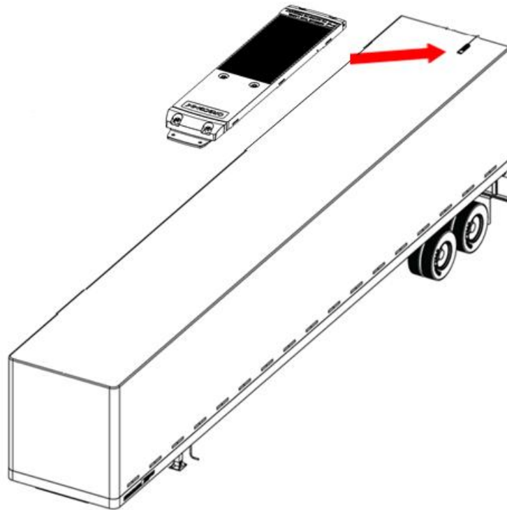
Figure 4: Rear Mounting Location on the Roof of a Trailer
