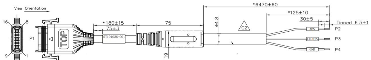
Figure 10: 16-PIN External Power Cable (units in mm)
