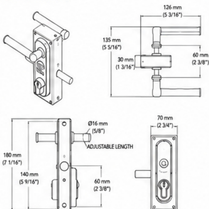
Dimension drawing:
