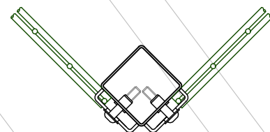
CORNER POST ARRANGEMENT
