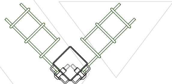
CORNER POST ARRANGEMENT
