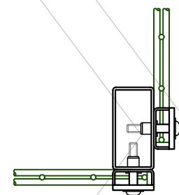
CORNER POST ARRANGEMENT
