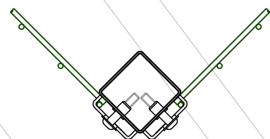
CORNER POST ARRANGEMENT
