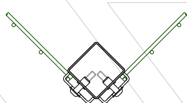
CORNER POST ARRANGEMENT
