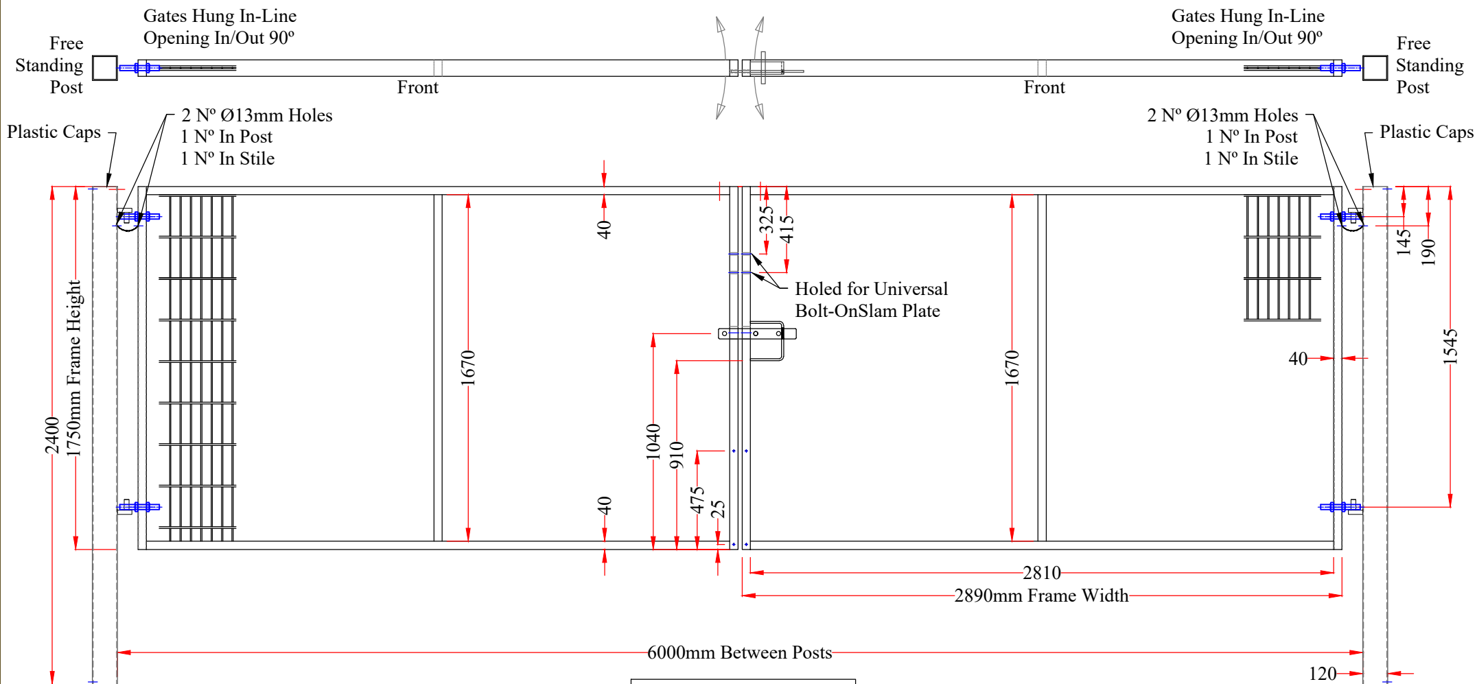
View of Front Elevation
