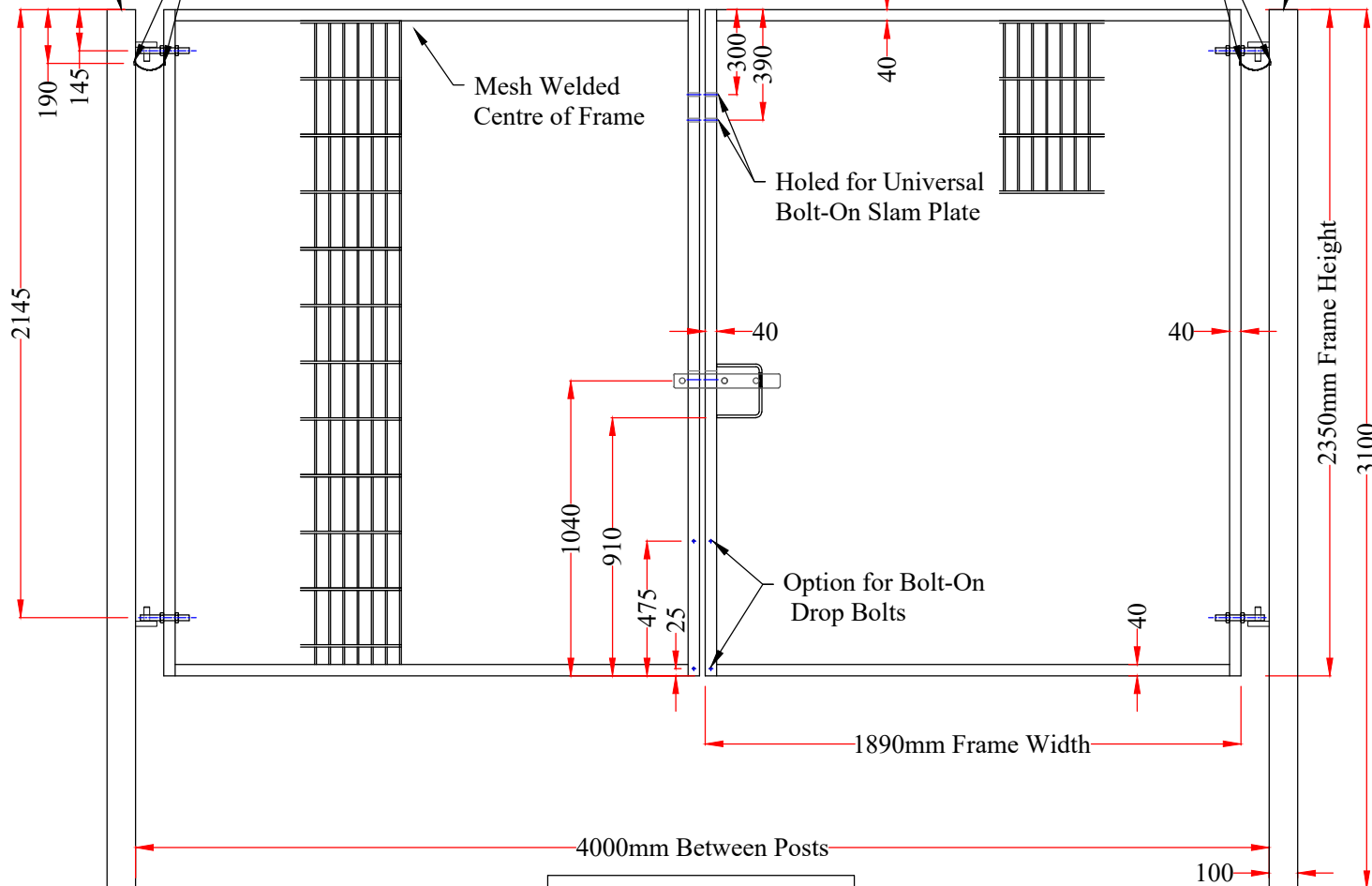
View of Front Elevation
