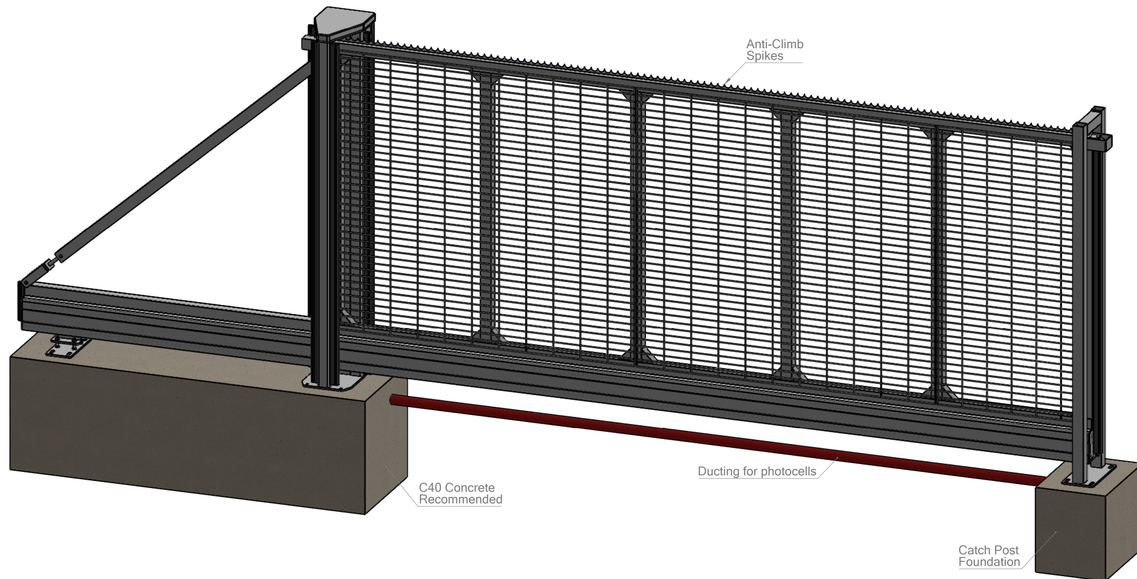
CLA FABRICATIONS - AUTO CANTILEVER SLIDING GATE 5000mm Opening x 2400mm High MESH INFILL - LEFT-HANDED GATE (viewed from outside site)
