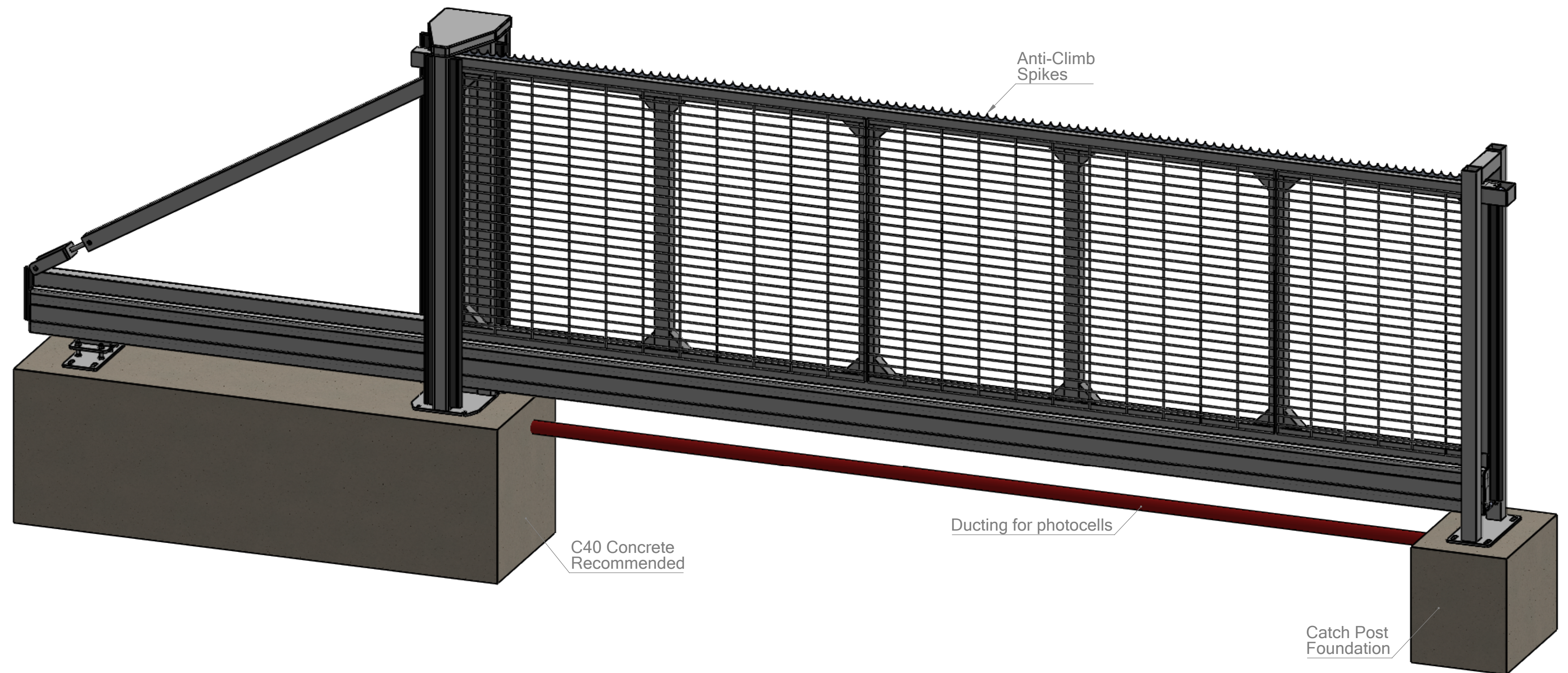
CLA FABRICATIONS - AUTO CANTILEVER SLIDING GATE 5000mm Opening x 1800mm High MESH INFILL - LEFT-HANDED GATE (viewed from outside site)
