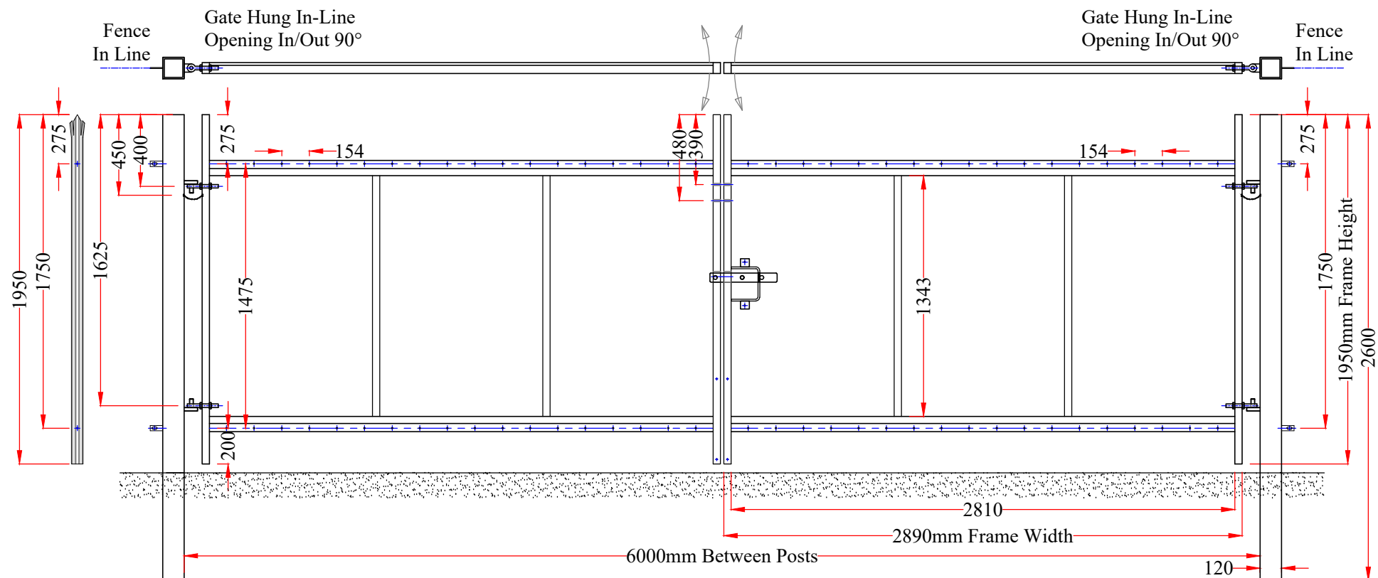
View of Front Elevation
