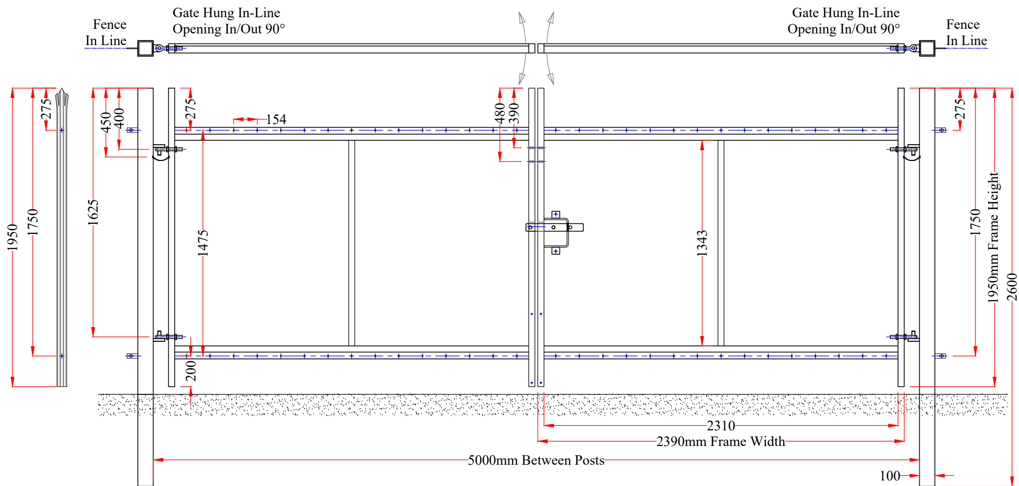
View of Front Elevation
