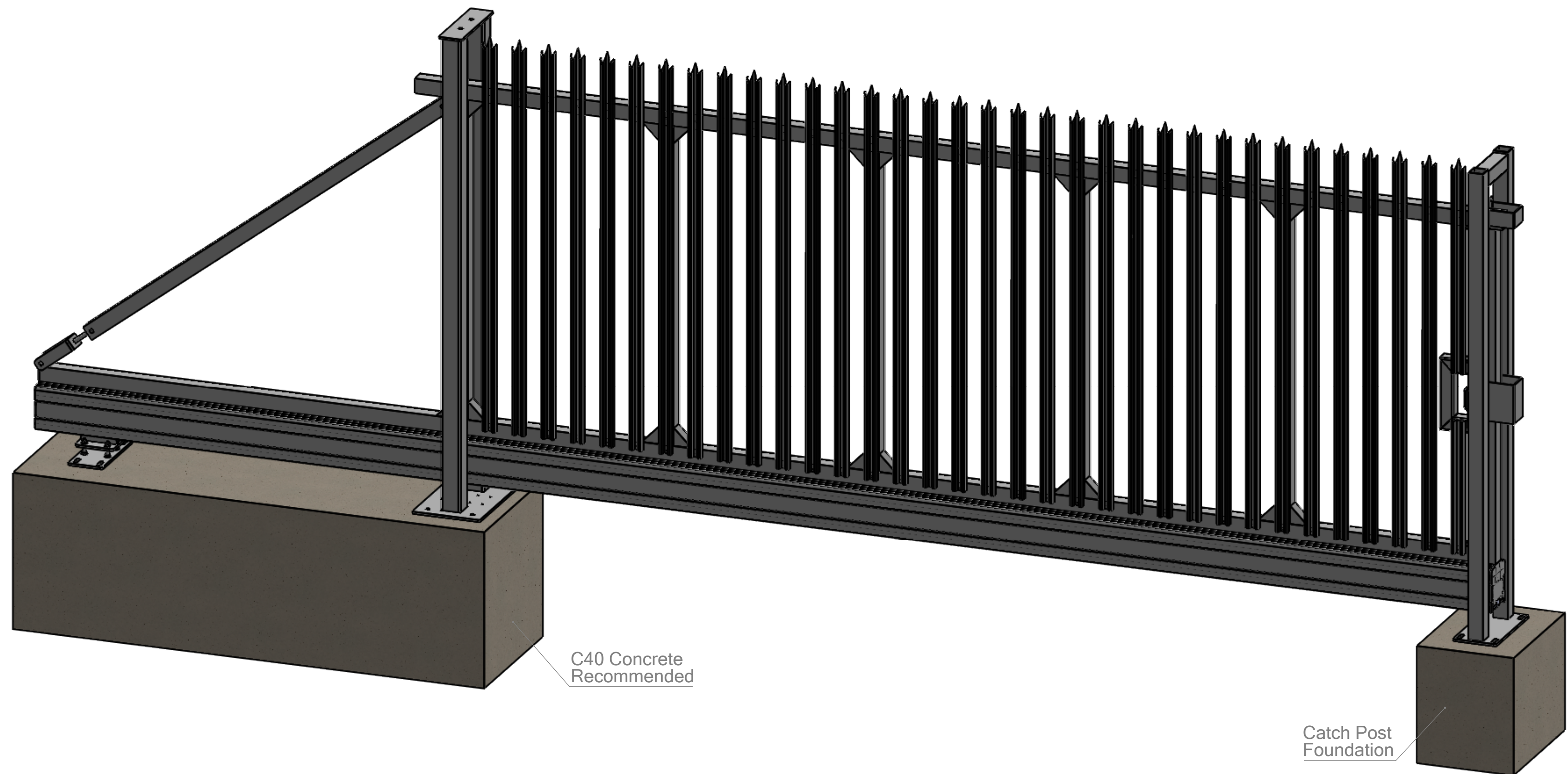
CLA FABRICATIONS - MANUAL CANTILEVER SLIDING GATE 5000mm Opening x 2400mm High PALISADE - LEFT-HANDED GATE (viewed from outside site)
