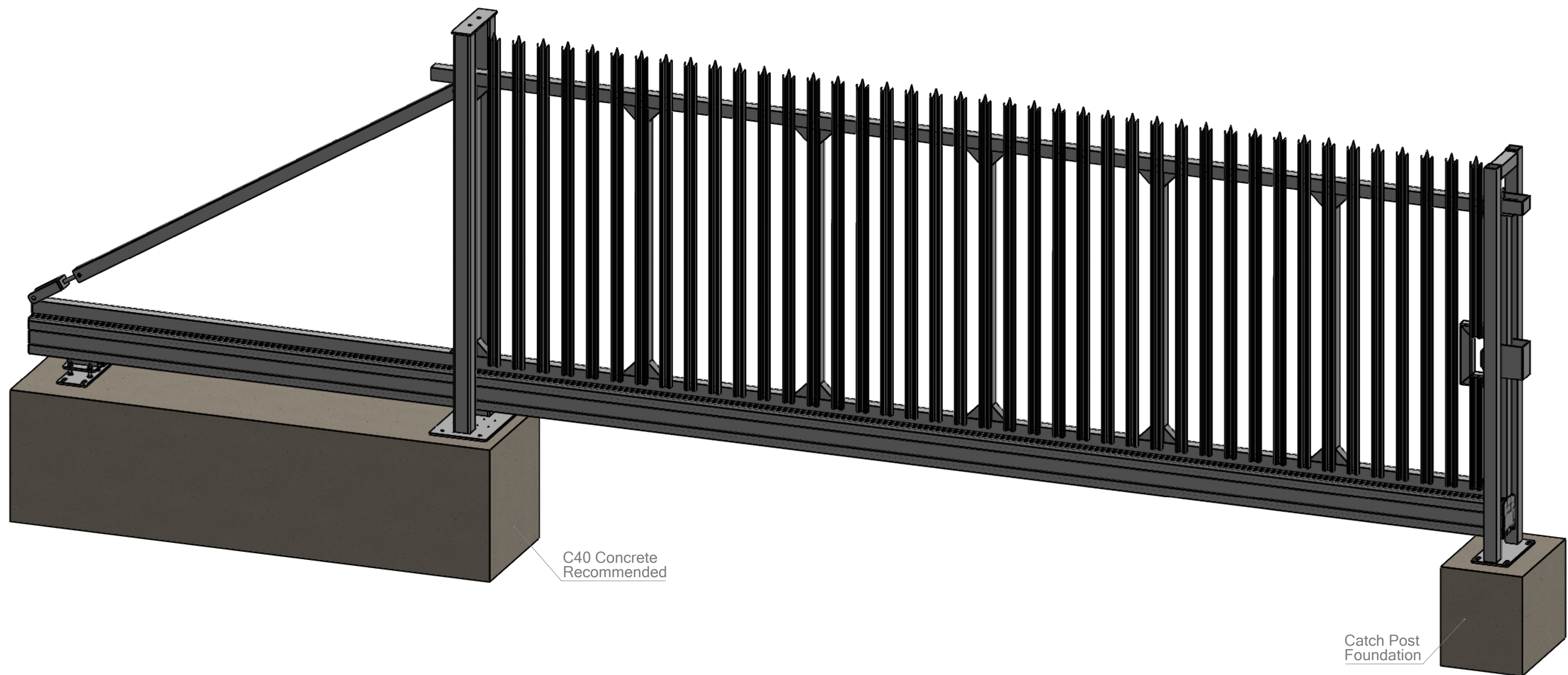
CLA FABRICATIONS - MANUAL CANTILEVER SLIDING GATE 6000mm Opening x 2400mm High PALISADE - LEFT-HANDED GATE (viewed from outside site)
