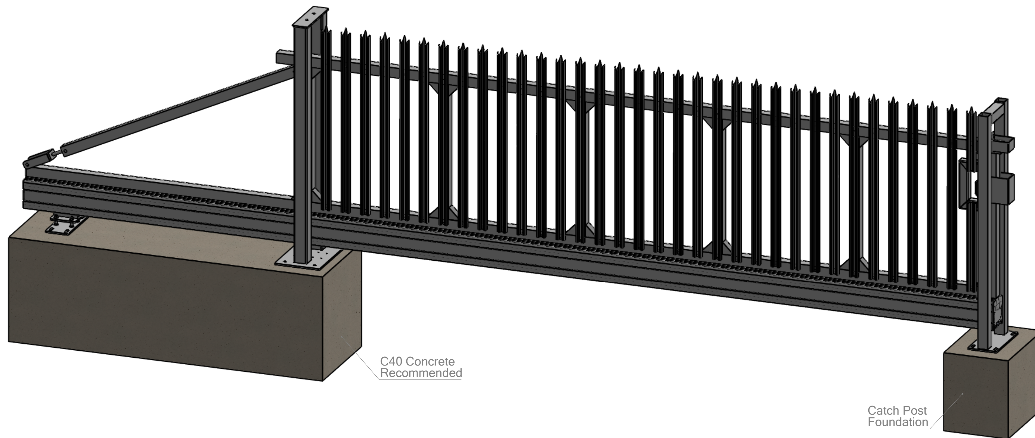
CLA FABRICATIONS - MANUAL CANTILEVER SLIDING GATE 5000mm Opening x 1800mm High PALISADE - LEFT-HANDED GATE (viewed from outside site)
