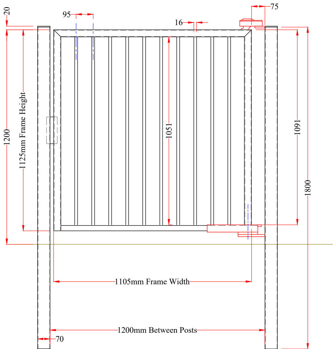
View of Front Elevation
