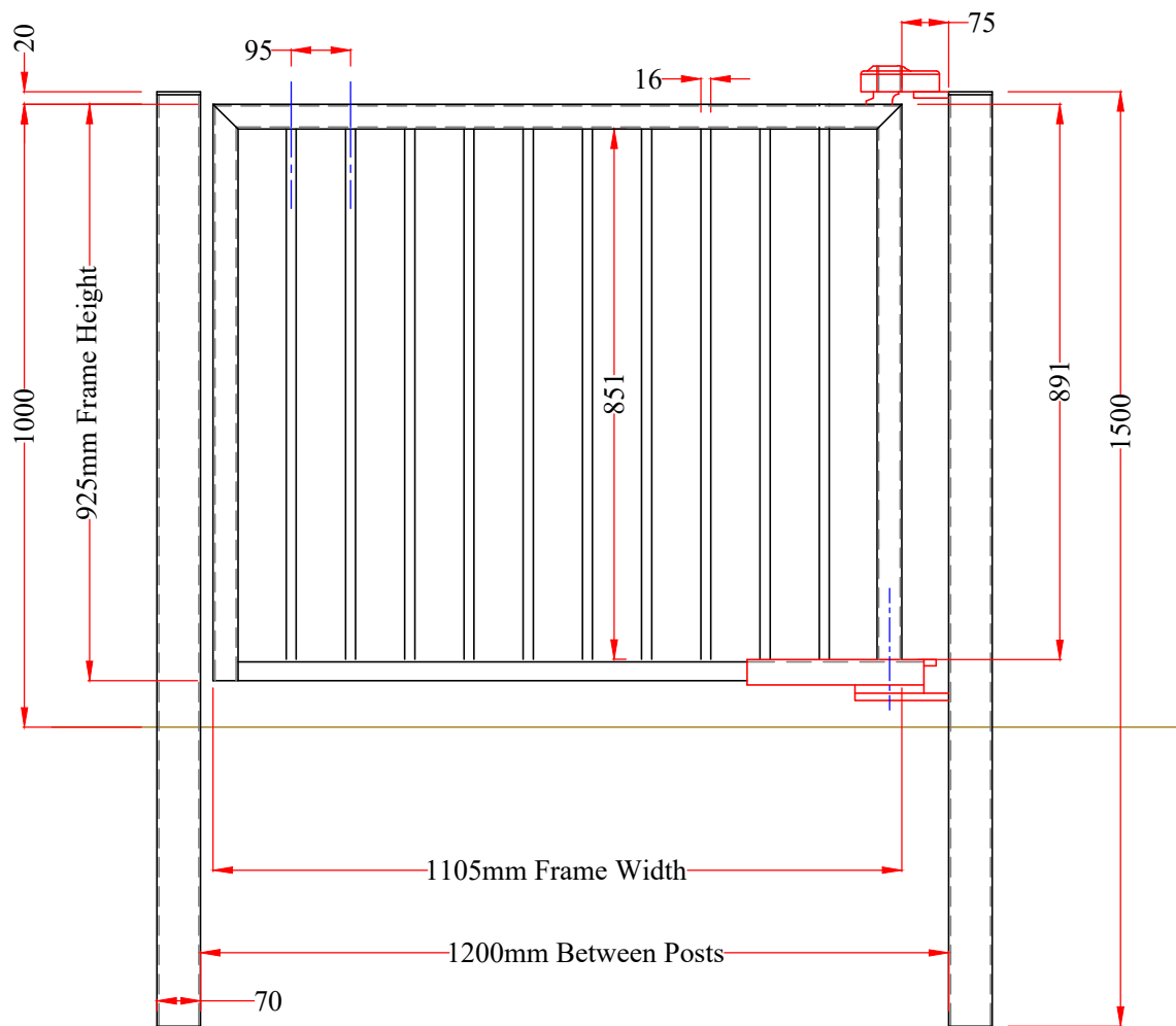
View of Front Elevation
