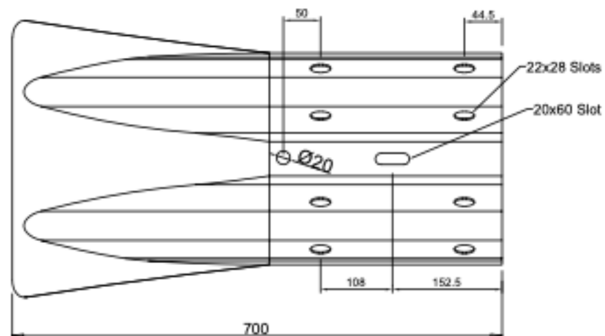
FACE VIEW
