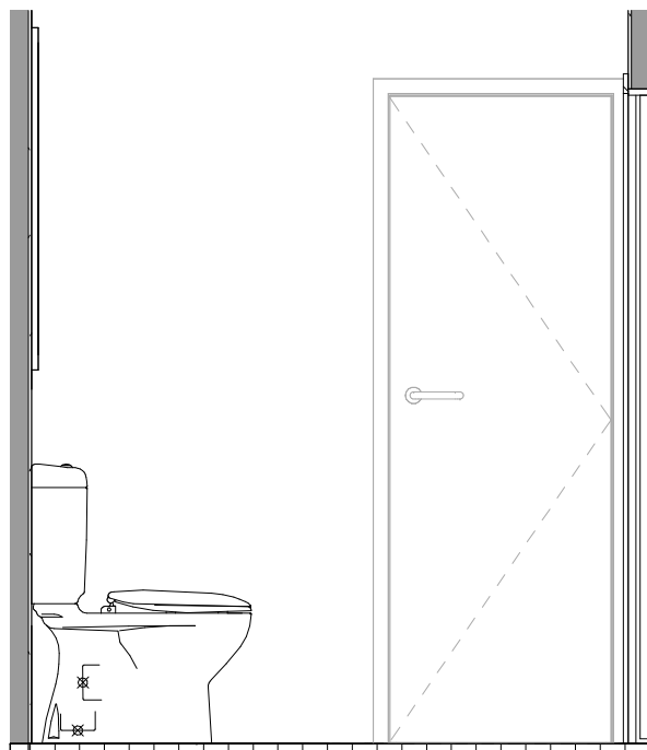
BATHROOM ELEVATION 4 1 : 25
