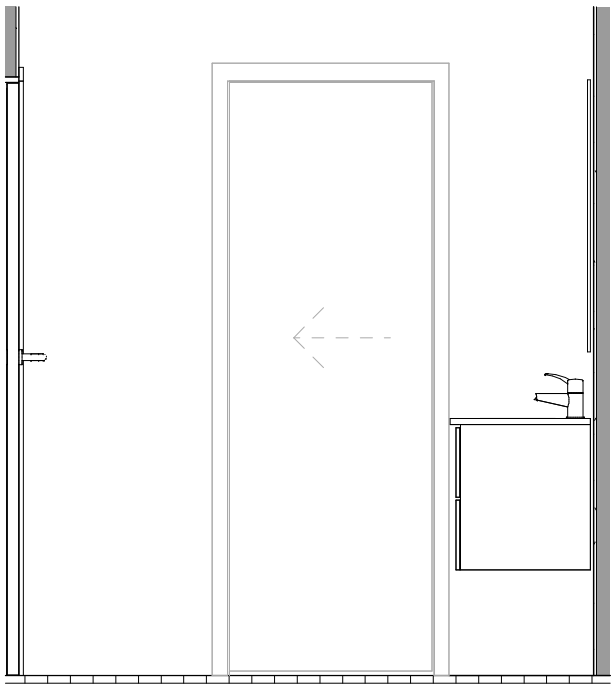
BATHROOM ELEVATION 1 1 : 25
