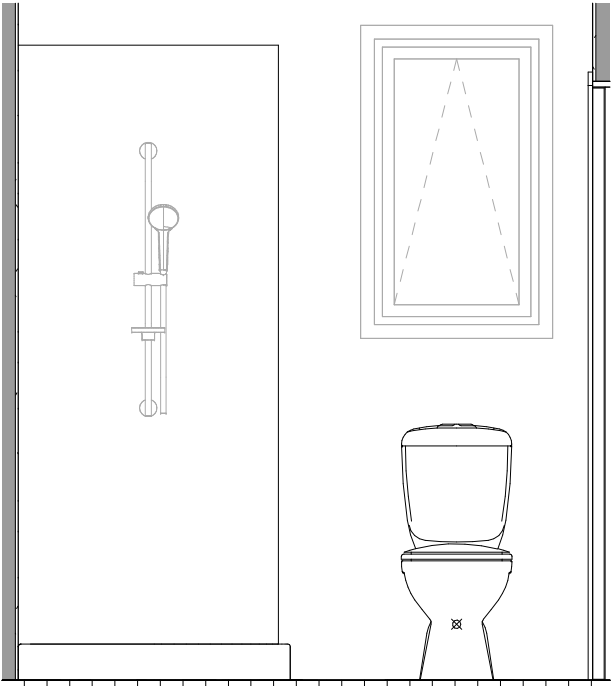
BATHROOM ELEVATION 3 1 : 25
