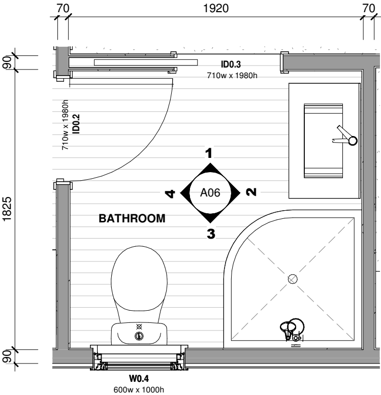
BATHROOM PLAN 1 : 25
