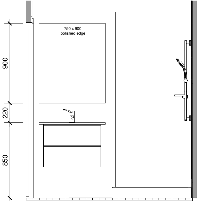
BATHROOM ELEVATION 2 1 : 25
