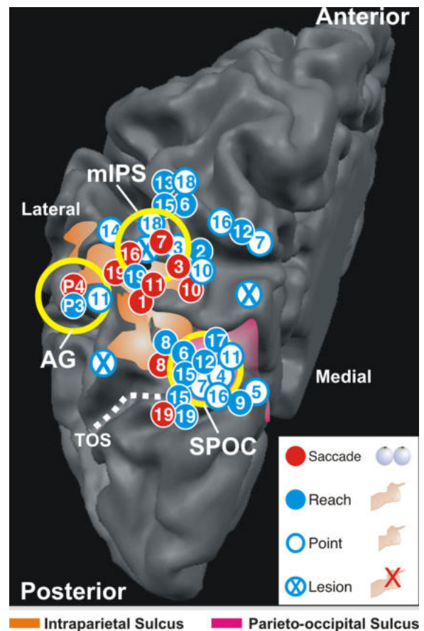
Figure 11. A comparison of fMRI, patient, and TMS studies. Three parietal sites were stimulated in current study (open yellow circles represent estimated stimulation areas): AG, mIPS, and SPOC, shown on a dorsomedial view of the left hemisphere. A summary of peak activation, lesion, and stimulation sites for saccade- (solid red circle), reach- (blue filled circle), and pointing-selective (open blue circle) regions identified in PPC by previous key studies in visuo-motor control is listed below. Note that foci were based on reported Talairach coordinates transformed to surface locations on a subject's pial surface and represent averaged group peaks of activity, lesion overlap, and stimulation area [shaded orange area, intraparietal sulcus; shaded magenta area, parieto-occipital sulcus; dotted white line, temporal occipital sulcus (TOS)]. fMRI activation, lesion foci, and TMS sites are as follows: for saccade, 1 (Serenio et al., 2001; Merriam et al., 2003), 8 (Schluppeck, 2005; Schluppeck et al., 2006), P4 (Elkington et al., 1992; Müri et al., 1996, 2000; Kapoula et al., 2001; Yang and Kapoula, 2004; Nyffeler et al., 2005); for saccade and reach, 8 (Levy et al., 2007), 19 (Beurze et al., 2009); for saccade and point, 3 (Medendorp et al., 2003), 7 (Zettel et al., 2007), 10 (Hagler et al., 2007), 11 (Fernandez-Ruiz et al., 2007), 16 (Tosoni et al., 2008); for reach, 2 (Pellijeff et al., 2006), 6 (Prado et al., 2005), 9 (Culham et al., 2008; Gallivan et al., 2009), 12 (Filimon et al., 2009), 13 (Beurze et al., 2007), 15 (Blangero et al., 2009), 17 (Busan et al., 2009a,b), P3 (van Donkelaar and Adams, 2005; Vesia et al., 2006, 2008; Koch et al., 2008); for point, 3 (Medendorp et al., 2005), 4 (Astafiev et al., 2003), 5 (Connolly et al., 2003), 14 (DeSouza et al., 2000); for eye-hand coordination, P3 (van Donkelaar et al., 2000); for joystick, P3 (Smyrnis et al., 2003), 18 (Grefkes et al., 2004); for lesion, X (Karnath and Perenin, 2005).
