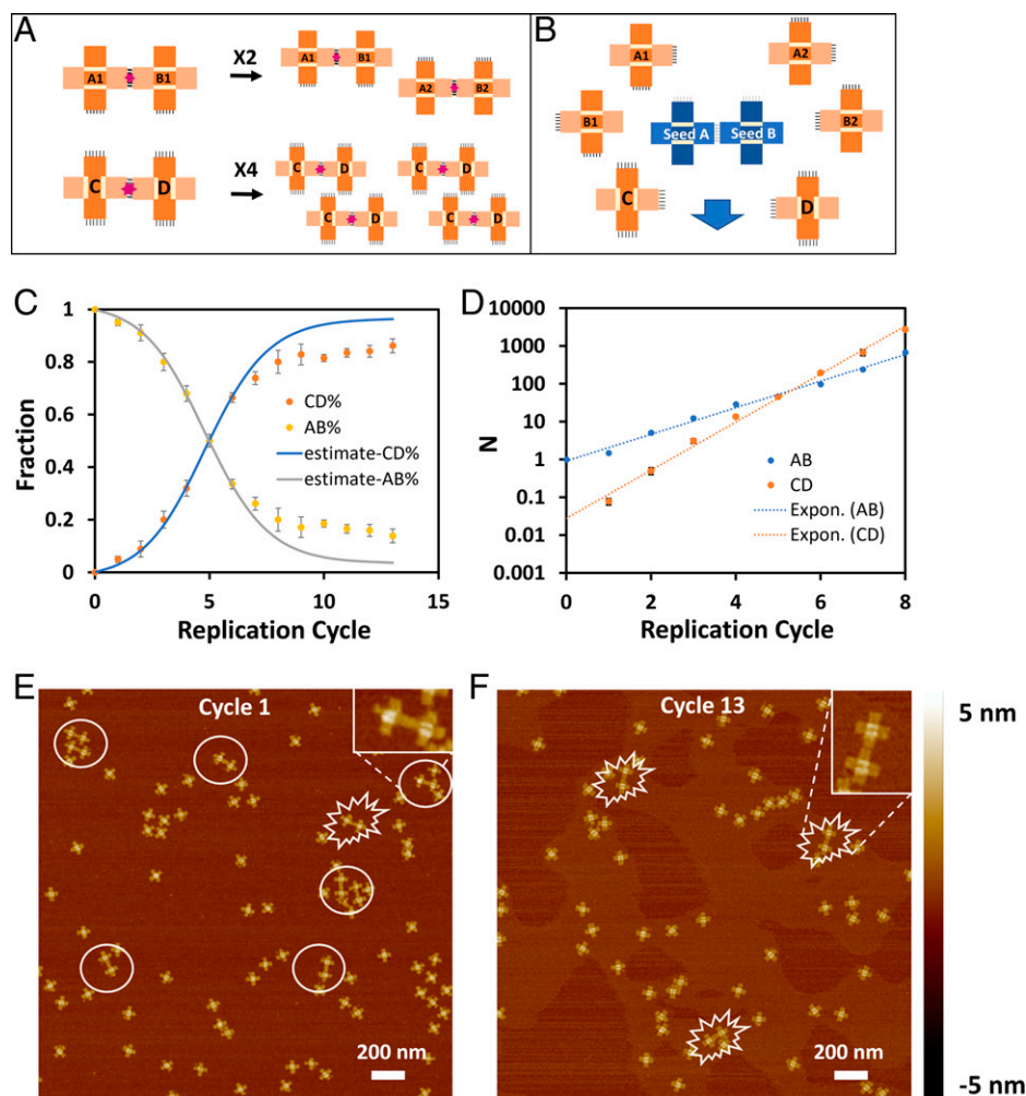
Fig. 4. (A) Schematic of two replication systems, A-B and C-D, with different replication rates. (B) Schematic of the mutation experiment starting with all four monomers and only A-B seed dimer. (C) The fraction of regular species (A-B) and mutated species (C-D) through 13 cycles of self-replication based on the counting of two species on AFM images. The solid line was the estimate of the species fraction based on the replication rate and the mutated self-assembly rate. (D) The natural logarithm numeral evolution of the two species through the first eight cycles of self-replication. (E and F) The representative AFM images of the sample after self-replication cycle 1 (E) and cycle 13 (F) show the change in the number of two species from five AB and one CD after cycle 1 to zero AB and three CD after cycle 13. The regular species are labeled with a circle and the mutated species are labeled with a 14-point explosion marker. The AFM sample are prepared at 48 °C to dehybridize the noncross-linked monomer. The 2.5- × 2.5-μm 2 representative AFM images were magnified from the 32- × 32-μm 2 whole image. The data in C come from imaging 1,635 “||||” and “=||” dimers from frames such as E and F.
