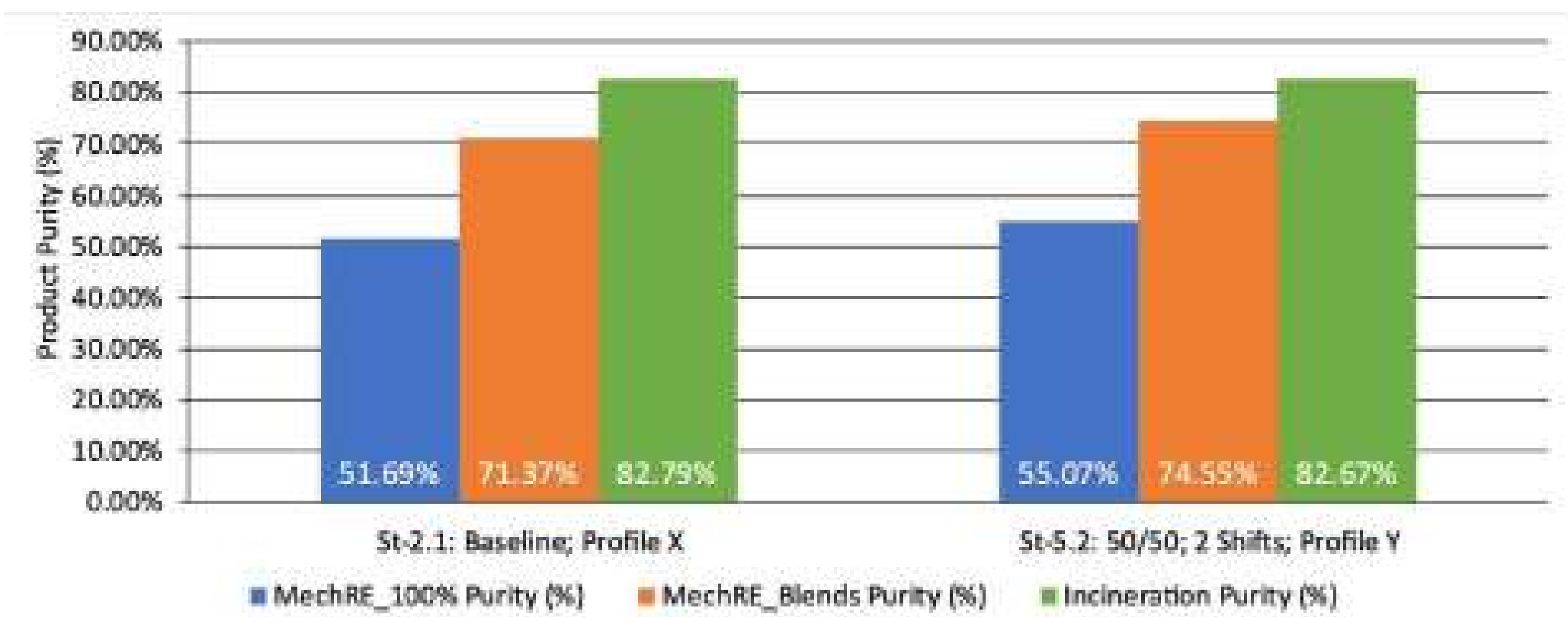
Figure 55: Product purity profile for S5.2 (2-shift, 50:50 blend) compared to baseline
