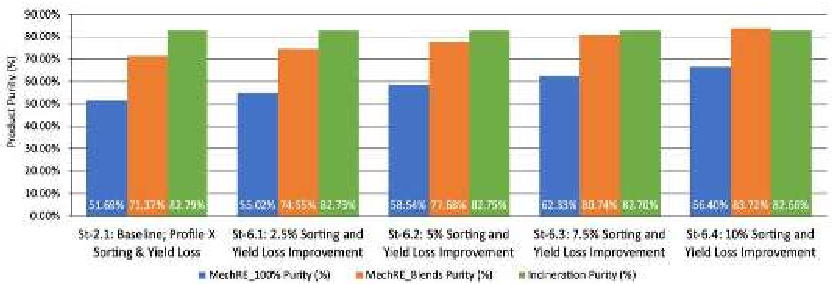
Figure 57: Product purity profile for S6.1 – S6.4 (2-shift, 50:50 blend) compared to baseline
