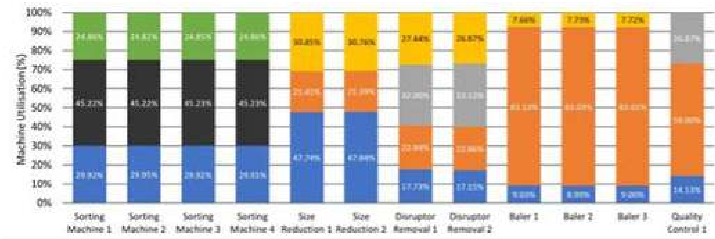
Figure 50: Individual machine utilisation profiles for the baseline (S2.1)
