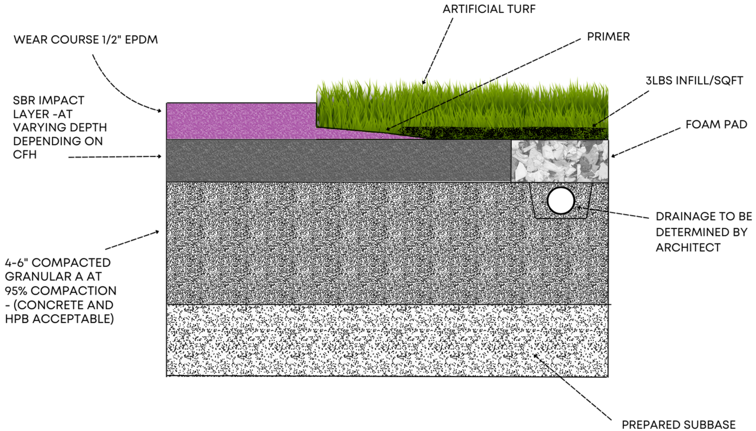
CROSS SECTION VIEW
