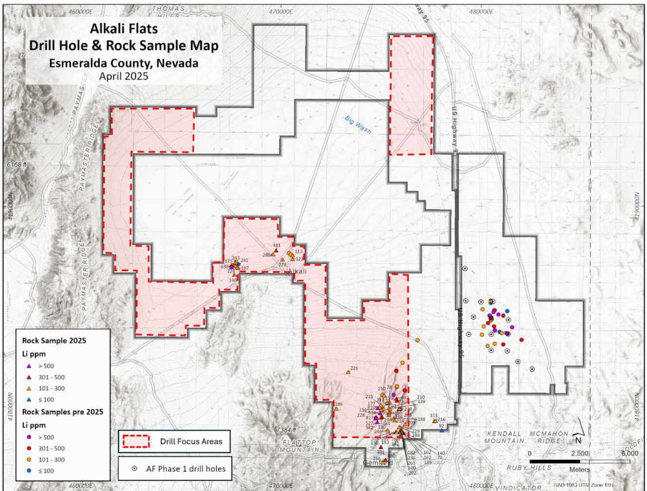
Figure 4. ALKALI FLATS 2025 SURFACE GEOLOGY MAPPING AND PHASE TWO DRILL FOCUS AREAS
