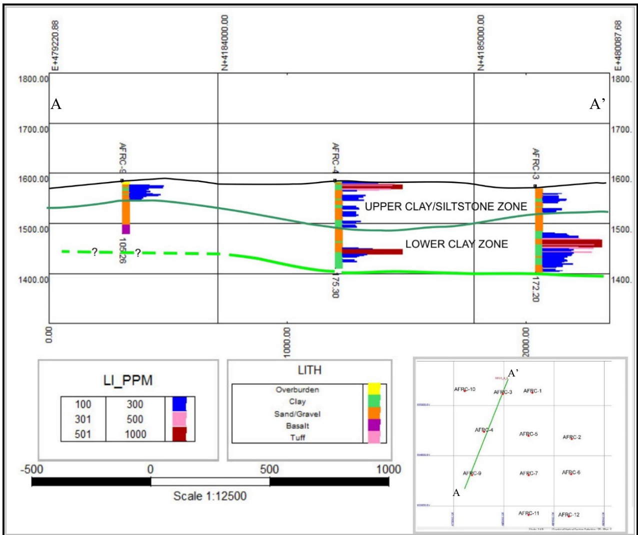
Figure 3. CROSS SECTION (A to A') OF SELECTED ALKALI FLATS PHASE 1 DRILL HOLES DISPLAYING INTERCEPTED LITHOLOGIES AND LITHIUM CONCENTRATION (15X VERTICAL EXAGGERATION)
